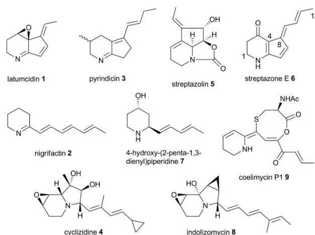
Figure 1. Structures of polyketide alkaloids from Actinobacteria.
