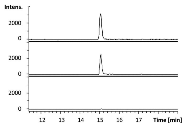
Figure 5. Extracted ion chromatograms at m/z = 130.1590 \pm 0.005 (corresponding to the [M+H]^+ ion for 21 ) from UHPLC-ESI-Q-TOF-MS analyses of an authentic standard of 21 (top), the CpkG-catalyzed reaction of 14 with L-alanine (middle) and a control reaction from which the enzyme was omitted (bottom).
