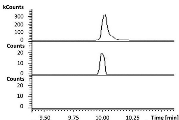
Figure 4. Extracted ion chromatograms at m/z = 187.2 (corresponding to the fragment ion of 16 resulting from loss of a methyl group) from GC-MS analyses of an authentic standard of 16 (top), the BSA-derivatized product of the CpkC-TR-catalyzed reduction of 13 with NADH (middle) and the BSA-derivatized product of a control reaction containing boiled enzyme (bottom).
