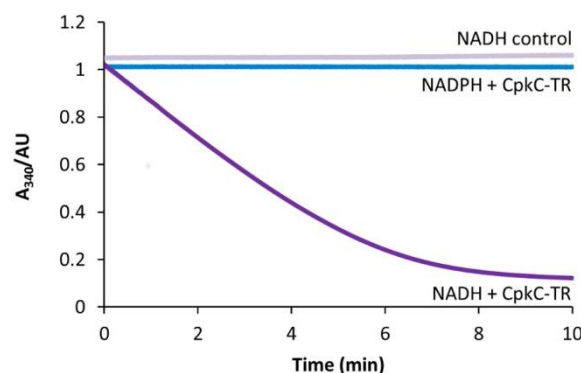
Figure 3. Analysis of NAD(P)H consumption in the CpkC-TR-catalyzed reduction of octanoyl-CoA using a continuous spectrophotometric assay.
