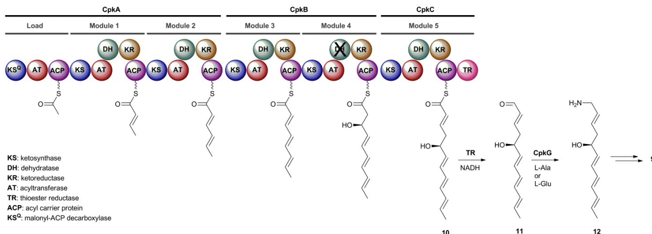
Figure 2. The proposed roles played by the CpkABC modular PKS and the CpkG \omega -transaminase in coelimycin P1 9 biosynthesis.
