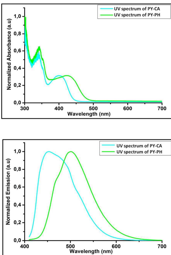
Figure 1. UV-vis absorption (upper) and photoluminescence (lower) spectra of PY-CA and PY-PH compounds in chloroform solution ( 1 \times 10^{-4} M). PL was measured at the 370 nm excitation wavelenght.
