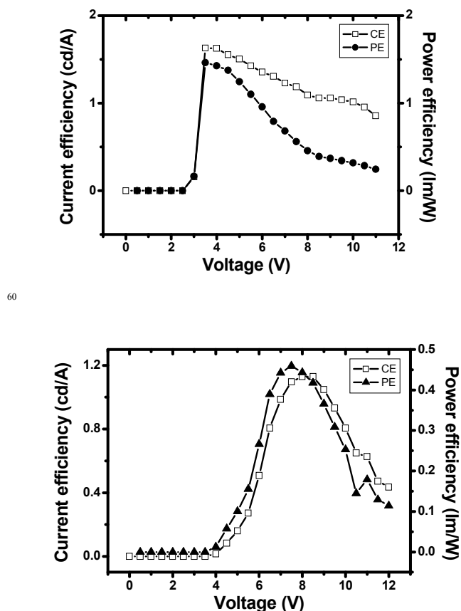
Figure 8. CE and PE characteristic of the PY-CA device (upper) and the PY-PH device (lower).
