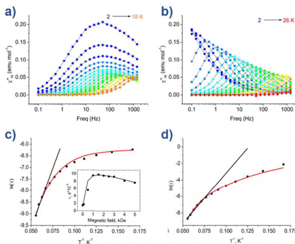
Fig. 14: Out-of-phase magnetic susceptibility for [\text{Co}(\text{Pzox})_3(\text{BC}_6\text{H}_5)]\text{Cl} ( 20 ) measured under; a) zero applied dc field and b) an applied dc field of 1500 Oe. c) Arrhenius plot of the natural log of the relaxation time vs. inverse temperature under a zero applied dc field and d) an applied dc field of 1500 Oe. Reprinted with permission from ref 43. Copyright (2015) American Chemical Society.
