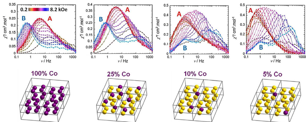
Fig. 23: Frequency dependent out-of-phase magnetic susceptibility ( \chi'' ) as a function of applied field (200 – 8200 Oe) at 2 K of [Co(DAPBH)(NO 3 )(H 2 O)] ( 67 ) magnetically diluted with [Zn(DAPBH)(NO 3 )(H 2 O)]. A and B represent two relaxation processes. Colour code: purple (Co) and yellow (Zn). Reprinted with permission from ref. 73. Copyright (2015) Royal Society of Chemistry
