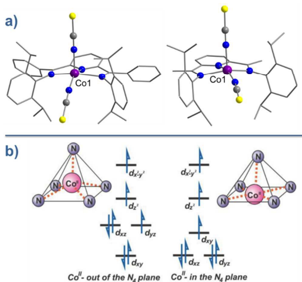
Fig. 16: a) Molecular structures of [\text{Co}(\text{LPh})(\text{NCS})_2] ( 25 , left) and [\text{Co}(\text{LMe})(\text{NCS})_2] ( 24 , right). Colour code: Purple (Co), blue (N), yellow (S), grey (C). b) d -orbital splitting diagrams for 24 and 25 , highlighting the effect of metal ion displacement from the basal plane. Reprinted with permission from ref. 47. Copyright (2011) American Chemical Society.
