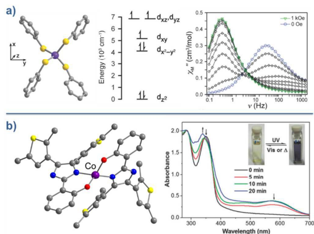
Fig. 18: a) Molecular structure, d -orbital splitting diagram and \chi'' vs. \nu plot as a function of H for [\text{Co}(\text{SePh})_4]^{2-} ( 32 ). Colour code: purple (Co), yellow (S), grey (C). Counter cation and hydrogen atoms omitted for clarity. Reprinted with permission from ref. 50. Copyright (2011) American Chemical Society. b) Molecular structure and absorption spectra changes under UV irradiation, thus demonstrating the photochromic behaviour of [\text{Co}(\text{hpbdti})_2] ( \text{hpbdtiH} = 2 -(2-hydroxyphenyl)-4,5-bis(2,5-dimethyl(3-thienyl))-1 H -imidazole) ( 37 ). Colour code: purple (Co), yellow (S), red (O), blue (N), grey (C). Hydrogen atoms omitted for clarity. Reprinted with permission from ref. 54a. Copyright (2013) Royal Society of Chemistry.
