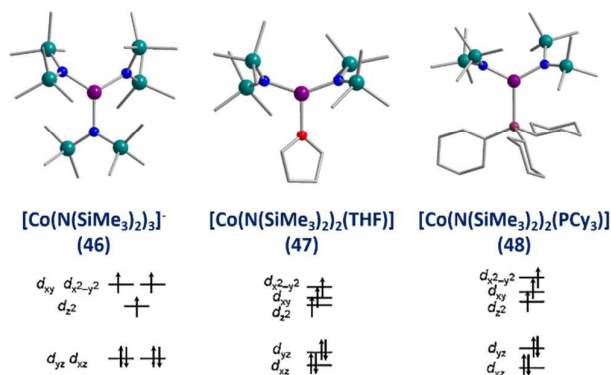
Fig. 19: Molecular structure and d -orbital splitting diagram for the three coordinate Co(II) complexes, [\text{Li}(15\text{-crown-5})][\text{Co}(\text{N}(\text{SiMe}_3)_2)_3] ( 46 ), [\text{Co}(\text{N}(\text{SiMe}_3)_2)_2(\text{THF})] ( 47 ) and [\text{Co}(\text{N}(\text{SiMe}_3)_2)_2(\text{PCy}_3)] ( 48 ). Colour code: purple (Co), plum (P), teal (Si), blue (N), red (O), grey (C). Hydrogen atoms omitted for clarity. Adapted with permission from ref. 56. Copyright (2014) American Chemical
