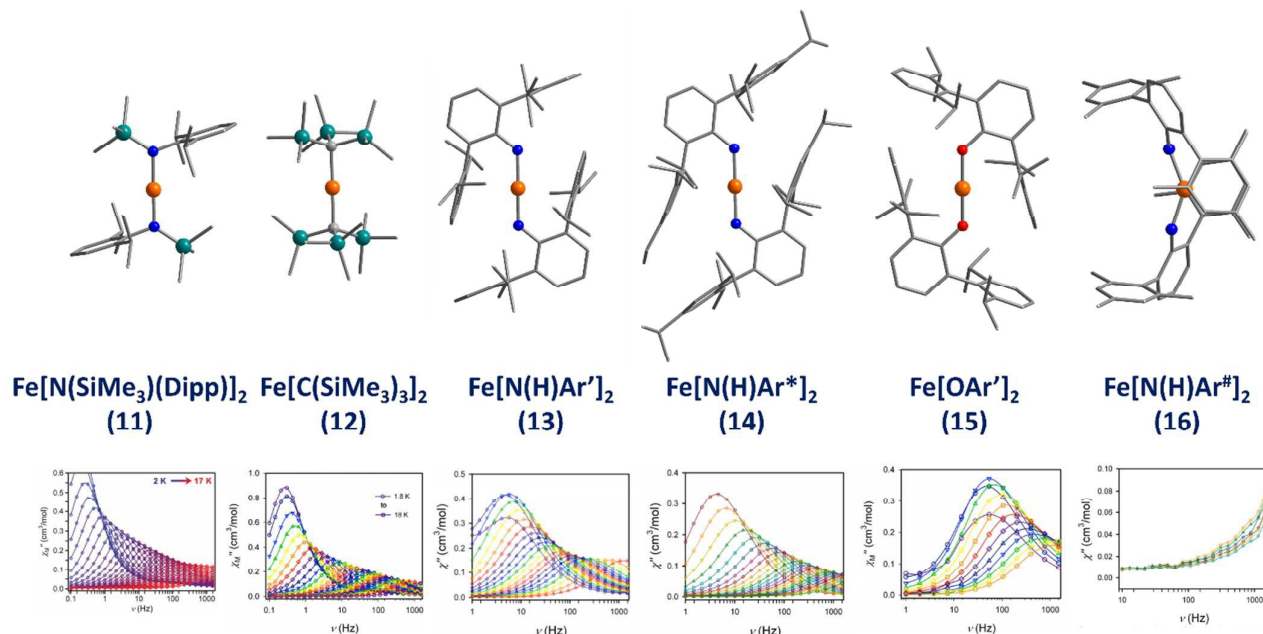
Fig. 11: Molecular structures of linear two coordinate Fe(II) complexes (from left to right): \text{Fe}[\text{N}(\text{SiMe}_3)(\text{Dipp})]_2 (11), \text{Fe}[\text{C}(\text{SiMe}_3)_3]_2 (12), \text{Fe}[\text{N}(\text{H})\text{Ar}' ]_2 (13), \text{Fe}[\text{N}(\text{H})\text{Ar}^*]_2 (14), \text{Fe}[\text{OAr}' ]_2 (15), and \text{Fe}[\text{N}(\text{H})\text{Ar}^\#]_2 (16). Colour code: orange (Fe), teal (Si), blue (N), red (O), grey (C). Hydrogen atoms omitted for clarity. Below is the frequency dependence of the out-of-phase magnetic susceptibility ( \chi'' ) as a function of temperature for each complex. Data were collected under applied dc fields of 500 Oe (11), 500 Oe (12), 875 Oe (13), 875 Oe (14), 2500 Oe (15), and 1000 Oe (16), respectively. Reprinted with permission from ref. 36b. Copyright (2013) Royal Society of Chemistry
