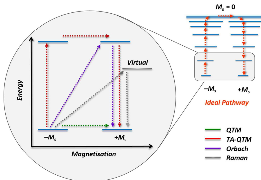
Fig. 2: Schematic representation of possible relaxation pathways in SMMs. Blue lines represent spin states. The grey line represents a virtual state by which Raman relaxation proceeds. Colour code: Green = ground state QTM, Red = thermally assisted QTM (TA-QTM), Purple = Orbach relaxation, Grey = Raman relaxation.
