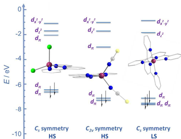
Fig. 17: Energy level diagram depicting selected \beta -spin frontier molecular orbitals of [Co(terpy)Cl 2 ] (C s symmetry) ( 26 ), [Co(terpy)(NCS) 2 ] (C 2v symmetry) ( 27 ) and [Co(terpy) 2 ] 2+ (C s symmetry). The increase in the number of \beta -spins for [Co(terpy) 2 ] 2+ comes at the cost of an \alpha -spin, resulting in an overall decrease in the molecular spin state. Reprinted with permission from ref. 48. Copyright (2013) Wiley-VCH.
