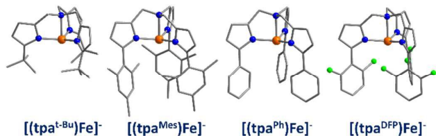
Fig. 9: Molecular structures of four coordinate trigonal pyramidal Fe(II) complexes of the form [(tpa R )Fe] + . Colour code: orange (Fe), green (Cl), blue (N), grey (C). Hydrogen atoms omitted for clarity.
