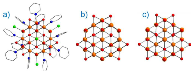
Fig. 3: a) Molecular structure of \text{Hpy}[\text{Fe}_{17}\text{O}_{16}(\text{OH})_{12}(\text{py})_{12}\text{Cl}_4]\text{Cl}_4 b) Metallic core of \text{Hpy}[\text{Fe}_{17}\text{O}_{16}(\text{OH})_{12}(\text{py})_{12}\text{Cl}_4]\text{Cl}_4 and c) A portion of the structure of magnetite demonstrating its similarities with \text{Hpy}[\text{Fe}_{17}\text{O}_{16}(\text{OH})_{12}(\text{py})_{12}\text{Cl}_4]\text{Cl}_4 . Colour code: orange (Fe), red (O), blue (N), green (Cl), grey (C). Hydrogen atoms omitted for clarity. Adapted from ref. 19.
