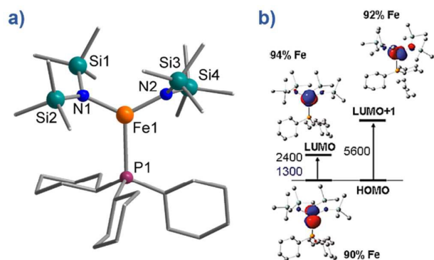
Fig. 10: a) Molecular structure of [\text{Fe}(\text{N}(\text{TMS})_2)_2(\text{PCy}_3)] , (TMS = \text{SiMe}_3 , Cy = cyclohexyl) (8). Colour code: orange (Fe), plum (P), teal (Si), blue (N), grey (C). Hydrogen atoms omitted for clarity. b) TD-DFT calculated excited states and \beta -spin molecular orbitals (MOs). The energies of the excited states and the metal contribution to the MOs are also shown. Reprinted with permission from ref. 34. Copyright (2011) American Chemical Society.
