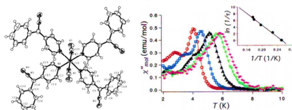
Fig. 12: Molecular structure of [\text{Co}(\text{SCN})_2(4\text{-dzbpy})_4] ( 18 ) (left) and out-of-phase magnetic susceptibility as a function of temperature (right), with an inset showing the Arrhenius fit of the data. Reprinted with permission from ref 39. Copyright (2003) American Chemical Society.
