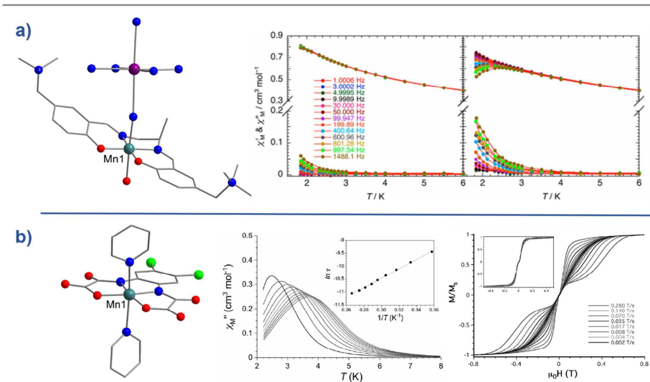
Fig. 20: a) Molecular structure of [Mn III (5-TMAM( R )-salmen)(H 2 O)(Co III (CN) 6 ) 2 ·7H 2 O·MeCN ( 49 ) Colour code: teal (Mn), purple (Co), blue (N), red (O), bright green (Cl), grey (C). Hydrogen atoms omitted for clarity. To the right of this, is the temperature dependence of the ac susceptibilities ( \chi' and \chi'' ) under an applied dc field of 4500 Oe and an ac field of 5 Oe. Reprinted with permission from ref. 57. Copyright (2013) American Chemical Society. b) Molecular structure of Ph 4 P[Mn(opbaCl 2 )(py) 2 ] ( 50 ). Colour code: teal (Mn), red (N), bright green (Cl), grey (C). Hydrogen atoms omitted for clarity. To the right of this, is the temperature dependence of the out-of-phase magnetic susceptibility ( \chi'' ) under an applied dc field of 1000 Oe and 4 Oe oscillating field (inset: Arrhenius plot), and, the sweep rate dependence of the magnetisation at 0.5 K (inset: at 0.03 K). Reprinted with permission from ref. 58. Copyright (2013) Wiley-VCH
