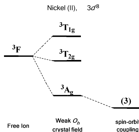
Fig. 6: Energy level diagram illustrating the effect of a weak octahedral crystal field and spin orbit coupling on the Ni(II) ion as described in the text. Levels expanded for clarity. The multiplicity of states arising from spin-orbit coupling are given in brackets.
