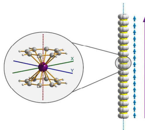
Fig. 5: A hypothesised chain-like arrangement of \text{M}(\text{COT})_2 monomers with uniaxial anisotropy, illustrating the concept of modular design of single-chain magnets. The axial anisotropy of each monomer is depicted as blue vectors and the vector addition of the monomeric axial anisotropies yields the net axial anisotropy (purple).
