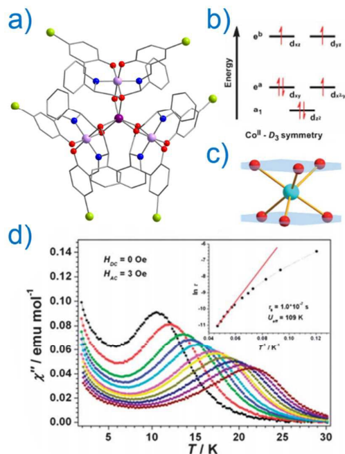
Fig. 13: a) Molecular structure of [\text{HNEt}_3][\text{Co}^{\text{II}}\text{Co}^{\text{III}}_3\text{L}_6] ( 19 ). Colour code: dark Purple (Co(II)), light purple (Co(III)), red (O), blue (N), grey (C) and light green (Br). Hydrogen atoms omitted for clarity. b) Simplified d -orbital splitting diagram c) Simplified coordination environment of central Co(II) ion and d) Out-of-phase magnetic susceptibility for 19 under zero applied dc field. Arrhenius plot of natural log of the relaxation time vs. inverse temperature as inset. Reprinted with permission from ref 42. Copyright (2013) Royal Society of Chemistry.
