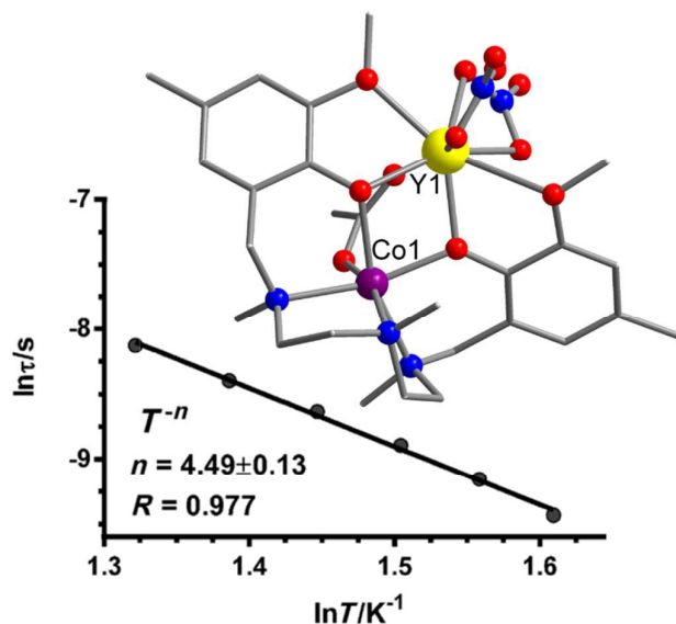
Fig. 22: Molecular structure of [\text{Co(L)(OAc)Y(NO}_3)_2] ( 65 ), with fitting of the relaxation time to a T^n power law as described in the text. Colour code: purple (Co), yellow (Y), blue (N), red (O), grey (C). Hydrogen atoms omitted for clarity. Reprinted with permission from ref. 71. Copyright (2013) Wiley-VCH.
