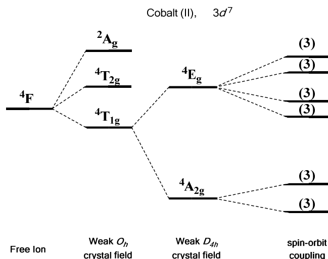
Fig. 7: Energy level diagram illustrating the effect of a weak octahedral crystal field and spin orbit coupling on the Co(II) ion as described in the text. Levels expanded for clarity. The multiplicity of states arising from spin-orbit coupling are given in brackets.
