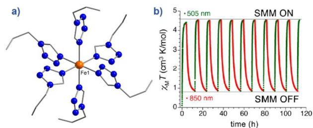
Fig. 8: a) Molecular structure of [\text{Fe}(\text{1-ptz})_6][(\text{BF}_4)_2] (2). Colour code: orange (Fe), blue (N), and grey (C). Hydrogen atoms omitted for clarity. b) Excitation and de-excitation cycling between the HS and LS configuration of 2, represented as a variation in the \chi_M T product at 10 K, under a 5000 Oe field. Reprinted with permission from ref. 28. Copyright (2013) American Chemical Society.
