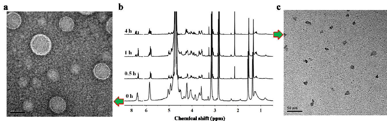
Fig. 4 Acid-triggered destabilization of supramolecular DOA:UPC liposomes. (a) Representative TEM image of negatively stained supramolecular DOA:UPC liposomes at pH 7.4 (Scale bars are 50 nm). (b) ^1\text{H} NMR spectra of supramolecular DOA:UPC liposome suspensions before and after incubation at pH 5.0 in \text{D}_2\text{O}/\text{HCl} (25 °C) for different period of time. From bottom to top: supramolecular liposome suspensions were incubated at pH 7.4 in \text{D}_2\text{O} and at pH 5.0 in \text{D}_2\text{O}/\text{HCl} for 0.5 h, 1 h and 4 h, respectively. The spectrum of the suspension at pH 7.4 is characterized by broad and featureless peaks. In contrast, the spectra after exposure to acidic stimuli are characterized by the sharpening and shifting of the peaks. (c) Representative TEM image of supramolecular DOA:UPC liposomes after incubation at pH 5.0 buffer for about 4 h (Scale bars are 50 nm).
