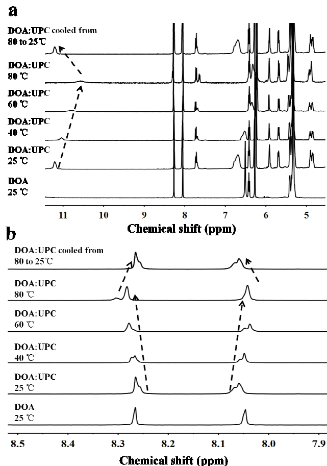
Fig. 2 Variable temperature ^1\text{H} NMR spectra of DOA and DOA:UPC. (a) ^1\text{H} NMR spectrum of DOA at 25 °C (bottom) and ^1\text{H} NMR spectra of DOA:UPC at 25 °C, 40 °C, 60 °C, 80 °C and cooled from 80 °C to 25 °C in the 4.5–11.5 ppm region. The arrow represents the changing trend of uracil NH chemical shift. (b) ^1\text{H} NMR spectrum of DOA at 25 °C (bottom) and ^1\text{H} NMR spectra of DOA:UPC at 25 °C, 40 °C, 60 °C, 80 °C and cooled from 80 °C to 25 °C in the 7.9–8.5 ppm region. The arrows represent the changing trend of adenine CH chemical shifts. The mixing ratio (DOA:UPC) was 1:1. Sample was allowed to equilibrate for 5 min at each temperature (1,1,2,2-tetrachloroethane- d_2 /dimethylsulfoxide- d_6 = 4/1).
