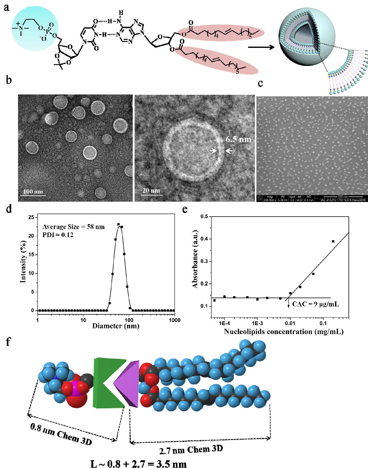
Fig. 3 Characterization of molecular self-assembly of supramolecular nucleoside phospholipids DOA:UPC. (a) Schematic representation of a supramolecular liposome self-assembled from the DOA:UPC nucleoside phospholipids. Supramolecular nucleoside phospholipids self-assemble into liposome-like bilayer structures in aqueous solution. (b) Representative TEM images of negatively stained supramolecular DOA:UPC liposomes. The liposome wall thickness is about 6.5 nm. (c) Representative SEM image of supramolecular DOA:UPC liposomes (Scale bars are 500 nm). (d) DLS profile for the supramolecular liposomes. (e) Relationship of the absorbance and the concentration of DOA:UPC in aqueous solutions. ( \lambda = 313 \text{ nm} , 25 \text{ }^\circ\text{C} ). (f) Estimation of the length of an extended DOA:UPC molecule according to the Chem3D results.
