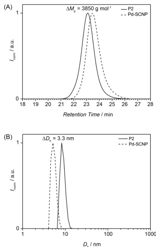
Fig. 2. SEC and DLS results of the Pd-SCNP formation. (A) Normalized SEC traces (DMAc, RI) of the linear precursor polymer P2 (solid line) and the Pd-SCNP (dashed line). (B) Number-averaged size distributions of the linear precursor P2 (solid line) and the Pd-SCNP (dashed line) in THF ( c = 4 mg/mL) at 25^\circ\text{C} .
