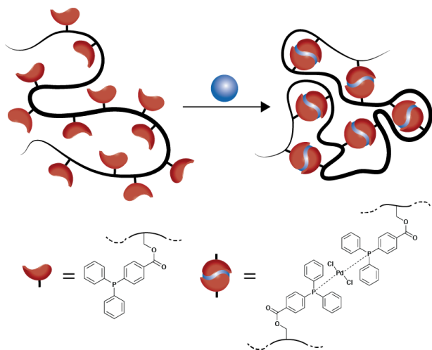
Scheme 1. Illustration of the Pd-SCNP formation via the intramolecular crosslinking of functional, linear precursor copolymers by metal-ligand complexation in diluted solution (schematic view, in which we suggest trans -configuration of the Pd-atoms, see text).
