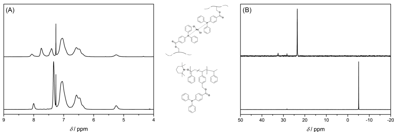
Fig. 1. Intramolecular crosslinking by metal-ligand complexation monitored by ^1\text{H} NMR (A) and ^{31}\text{P}\{^1\text{H}\} NMR spectroscopy (B) in \text{CDCl}_3 at 25^\circ\text{C} . The complete shift of the proton and phosphorus resonances indicates quantitative complexation. (The crosslinking chemistry presents a schematic view, in which we suggest a trans -configuration of the Pd-atoms, see text).
