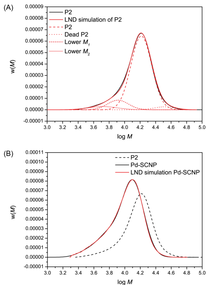
Fig. 4. Experimental SEC (DMAc, RI) data and corresponding log-normal distribution (LND) simulations. (A) Black trace: experimental P2 , red trace: LND fit of P2 using 4 distributions, namely P2 (red dashed), dead P2 (red dotted), lower M_1 (red short dashed), and lower M_2 (red short dotted). (B) Black trace: experimental Pd-SCNP , red trace: LND fit of Pd-SCNP using 7 distributions, black dashed trace: experimental P2 for comparison.
