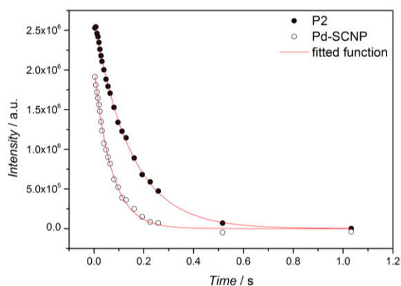
Fig. 3. T_2 decay curves for the methylene bridge protons of the linear precursor polymer P2 (dots) and the Pd-SCNP (open dots). The red curves represent mono exponential decay functions that have been fitted to the data points.
