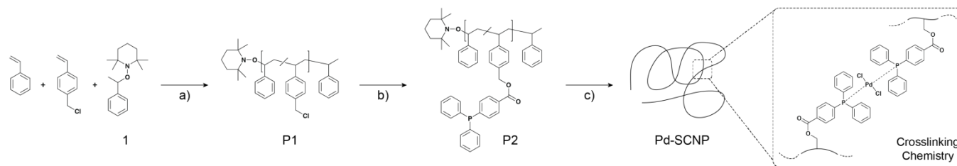
Scheme 2. Synthetic strategy for the preparation of palladium(II) crosslinked single-chain nanoparticles (Pd-SCNPs). a) bulk, 125 °C, 5h; b) 4-(diphenylphosphino)benzoic acid, K 2 CO 3 , DMF (dry), 50 °C, 16 h; c) Pd(COD)Cl 2 , DCM (dry), a.t., 21 h. (The crosslinking chemistry presents a schematic view, in which we suggest a trans -configuration of the Pd-atoms, see text).
