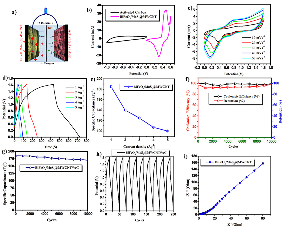
Fig. 7 (a) Schematic representation of the assembled \text{BiFeO}_3/\text{MoS}_2@\text{MWCNT} // \text{AC} asymmetric supercapacitor; (b) comparative cyclic voltammetry curves of \text{BiFeO}_3/\text{MoS}_2@\text{MWCNT} and AC electrodes at 10\ \text{mV s}^{-1} ; (c) CV profiles of the full asymmetric device at various scan rates; (d) Galvanostatic charge–discharge profiles of the ASC device; (e) C_s at different current densities; (f) capacitance retention and Coulombic efficiency over 10 000 cycles; (g) specific capacitance evolution during the cycling testing; (h) charge–discharge profiles for the initial 250 cycles; (i) electrochemical impedance spectroscopy analysis of the ASC device.
