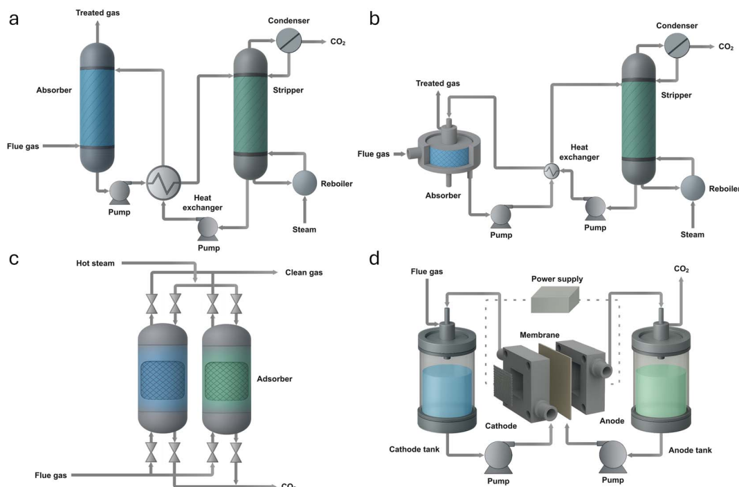
Fig. 20 General process schematics of representative \text{CO}_2 capture contactors and reactor configurations: (a) packed-bed scrubber (absorption column), (b) RPB absorber, (c) fixed-bed adsorber, and (d) electrochemical flow cell for \text{CO}_2 capture/conversion.
