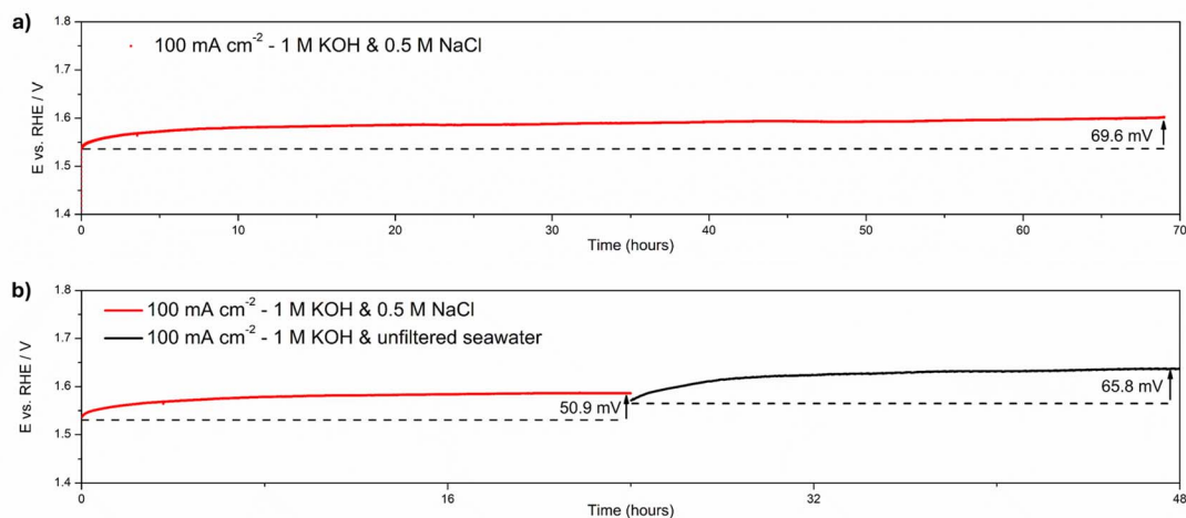
Fig. 6 (a) CP stability test in 1 M KOH & 0.5 M NaCl at 293 K at a constant current of 100 \text{ mA cm}^{-2} for 70 hours using \text{NiFe}(\text{OH})_2 coated at 250 \text{ mA cm}^{-2} on a Ni microelectrode (b) comparison of \text{NiFe}(\text{OH})_2 at a constant current of 100 \text{ mA cm}^{-2} in 1 M KOH & 0.5 M NaCl and 1 M KOH & unfiltered seawater at 293 K on a Ni microelectrode, tests were conducted separately with a new sample made for each experiment.
