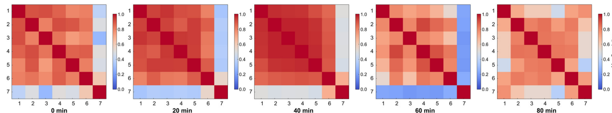
Fig. 3 Two-dimensional distribution of the cross-correlations at zero lag time G(0) . Numbers along the x and y coordinates represent the seven microspheres of interest (P1–7). Color bar indicates the value of G(0) .
