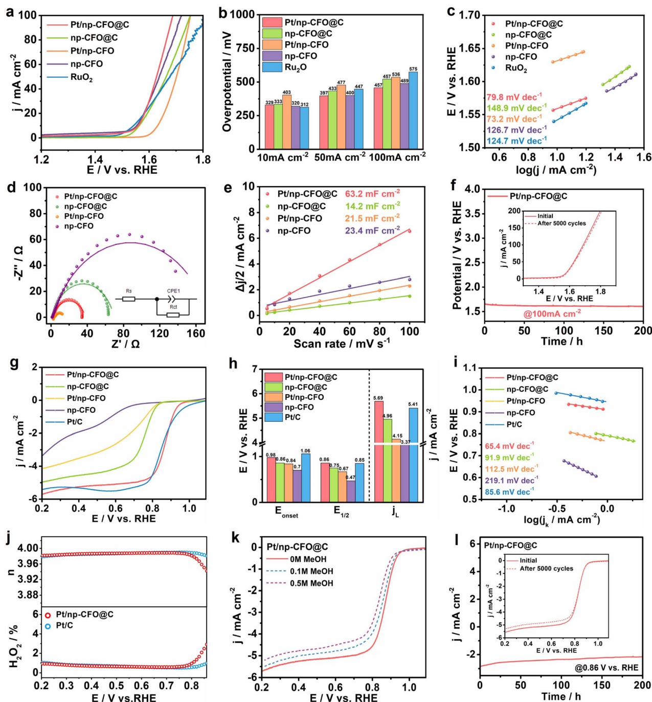
Fig. 4 OER performances: (a) LSV curves; (b) a comparison of \eta_{10} , \eta_{50} and \eta_{100} ; (c) Tafel slopes; (d) Nyquist plots; (e) C_{dl} values; and (f) the CP profile at 100 mA cm -2 ; the inset shows LSV curves of Pt/np-CFO@C before and after ADT. ORR performances: (g) LSV curves; (h) a comparison of E_{onset} , E_{1/2} and j_L ; (i) Tafel slopes; (j) electron transfer numbers and H 2 O 2 yields on Pt/np-CFO@C and Pt/C derived from RRDE testing; (k) methanol tolerance of Pt/np-CFO@C; and (l) the CA profile at 0.86 V vs. RHE; the inset shows LSV curves of Pt/np-CFO@C before and after ADT.
