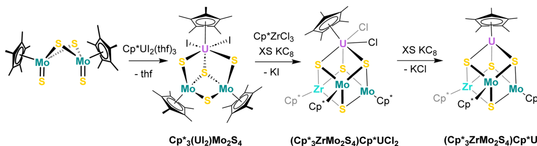
Scheme 2 Syntheses of \text{Cp}^*_3(\text{U})\text{Mo}_2\text{S}_4 , (\text{Cp}^*_3\text{ZrMo}_2\text{S}_4)\text{Cp}^*\text{UCl}_2 , and (\text{Cp}^*_3\text{ZrMo}_2\text{S}_4)\text{Cp}^*\text{U} .
