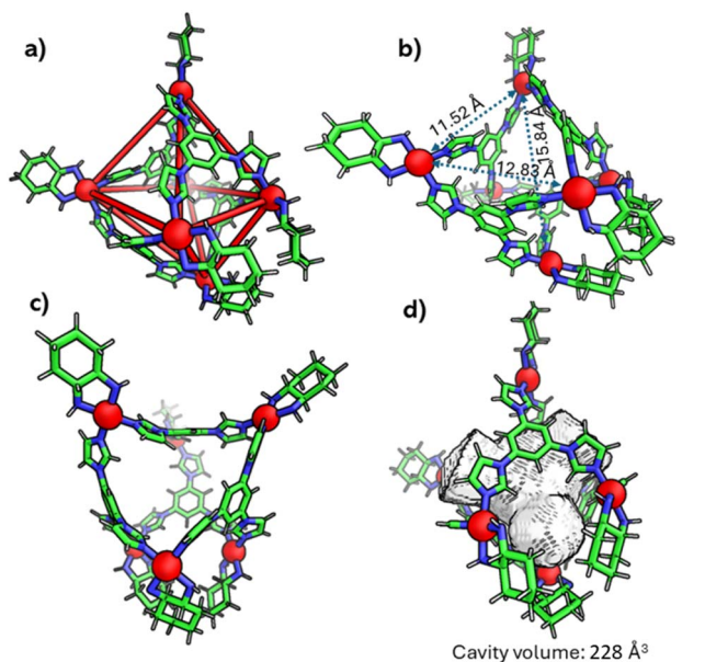
Fig. 3 X-ray crystal structure of \text{C}_1 (CCDC no. 2455229). (a) Distorted octahedral shape of the cage; (b and c) side views of the cage and (d) cavity space of the cage (colour codes: C, green; N, blue; and Pd, red).
