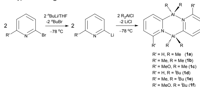
Scheme 3 Synthesis of Al(III) dimers of the type (2-py' = 6-substituted pyridyl), the precatalysts used in polymerisation and cyclotrimerisation in the current study, including the compound numbering scheme.
