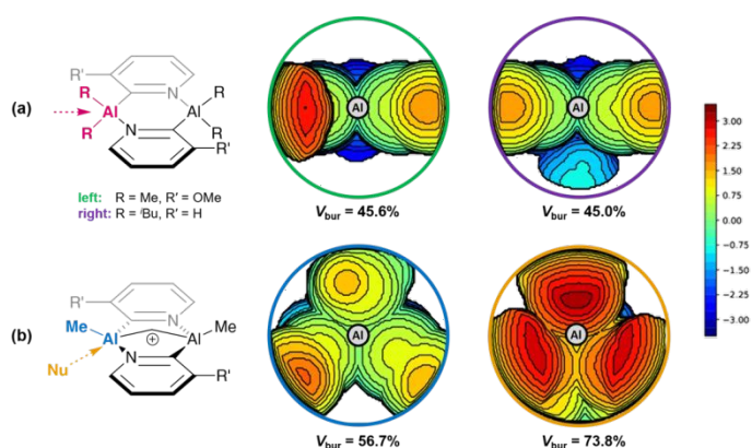
Figure 12 Topographic steric maps showing the steric pressure exerted on each aluminium centre: (a) by the ring system in the neutral pre-catalysts 1c and 1d (left and right, respectively; viewed on the plane of the ring from the direction of the alkyl groups); (b) by the ring system in the active cationic catalyst 2a (viewed from the direction of the terminal methyl) (left) or by the entire ligand scaffold (including terminal alkyls, viewed from the direction of the incoming substrate) (right). The scale of the isocontours of altitude from the Al centre range between \pm 3.5 \text{ \AA} .
