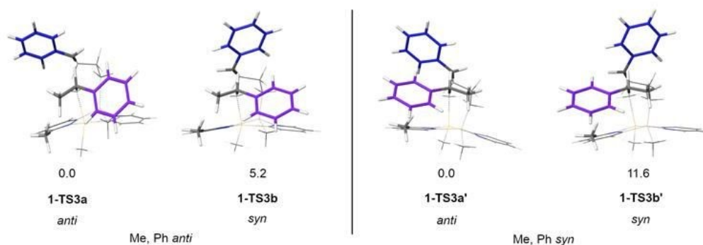
Figure 11 The four isomeric model transition states studied. Values given are relative Gibbs free energies in \text{kJ mol}^{-1} . Absolute stereochemistry is labelled by relation of Me on catalyst and Ph on chain (purple) in conformation when H projects into other chain.
