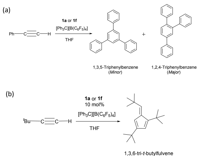
Scheme 4 Products of the reactions of (a) phenylacetylene, and (b) t -butylacetylene with 1a or 1f /[Ph 3 C][B(C 6 F 5 ) 4 ].
