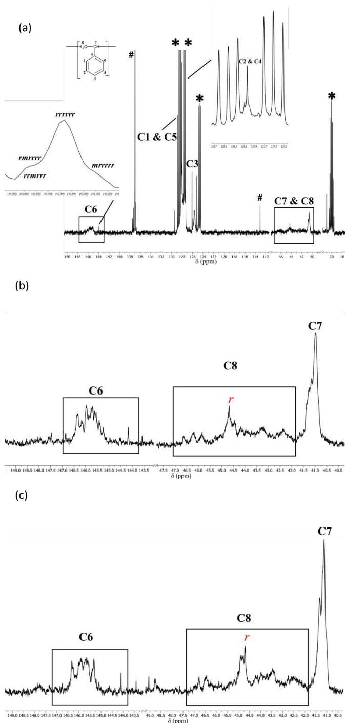
Figure 3 (a) ^{13}\text{C} NMR (25 °C, d_8 -toluene, 126 MHz) spectrum of atactic + syndiotactic polystyrene prepared using 0.5 mol% catalytic loading of precatalyst 1e and [\text{Ph}_3\text{C}][\text{B}(\text{C}_6\text{F}_5)_4] at -15 °C depicting the signals for the aromatic ipso carbon and the methylene carbon. The broad signals for C6 and C8 represent the atactic component, while the sharper peaks represent the syndiotactic component. The sharp signal labelled with a red r marks the signal depicting a 100% probability of having r diads. 21,32 The signals marked as # can be best attributed to unreacted [\text{Ph}_3\text{C}][\text{B}(\text{C}_6\text{F}_5)_4] , remnant toluene or potentially any unreacted styrene. * d_8 -toluene. (b) ^{13}\text{C} NMR (100 °C, d_2 -tetrachloroethane, 126 MHz, 1000 scans) showing the signals for the ipso carbon C6 and the methylene carbon C8. The sharp signal labelled with a red r marks the signal depicting a 100% probability of having r diads. 21,32 (c) ^{13}\text{C} NMR (100 °C, d_4 - o -dichlorobenzene, 126 MHz, 1000 scans) showing the signals for the ipso carbon C6 and the methylene carbon C8. The sharp signal labelled with a red r marks the signal depicting a 100% probability of having r diads. 21,32
