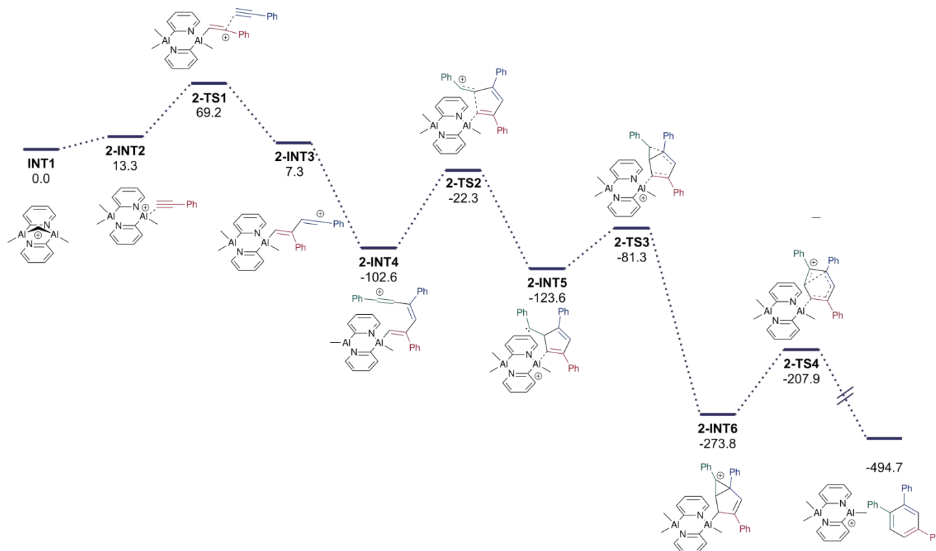
Figure 13 Proposed reaction mechanism and energy profile diagram of the calculated trimerisation reaction pathway (Gibbs free energies in kJ mol -1 ).
