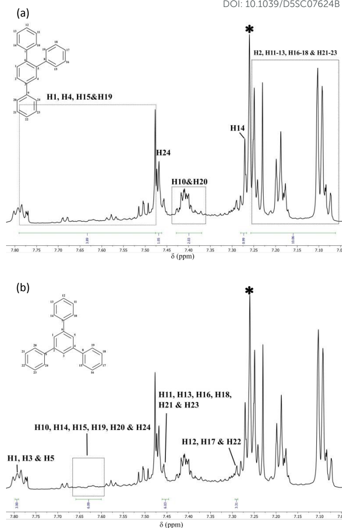
Figure 6. The spectra in (a) and (b) are duplicated here, to allow presentation of the assignments for both isomers more clearly. (a) 1 H NMR (25 °C, d -chloroform, 700 MHz) spectrum of a mixture of 1,2,4- and 1,3,5-triphenylbenzene prepared using a 0.5 mol% precatalyst loading of 1f and [Ph 3 C][B(C 6 F 5 ) 4 ] (cation 2f ) at room temperature, with the resonances for the 1,2,4-isomer highlighted. (b) The same spectrum with the resonances for 1,3,5-triphenylbenzene highlighted. * d -chloroform.
