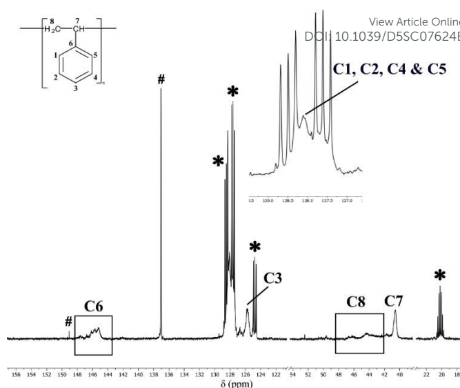
Figure 2 13 C NMR (25 °C, d 8 -toluene, 126 MHz) spectrum of atactic polystyrene prepared using a 0.5 mol% precatalyst loading of 1a and [Ph 3 C][B(C 6 F 5 ) 4 ] at room temperature. The resonances are broad and overlapping and have been assigned based on existing literature. 21,30,31 The signals marked as # can be best attributed to unreacted [Ph 3 C][B(C 6 F 5 ) 4 ], remnant toluene or potentially any unreacted styrene. * d 8 -toluene.
