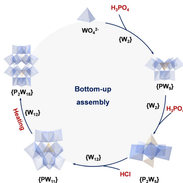
Fig. 4 Bottom-up assembly route from WO 4 2- to {P 2 W 18 }.
