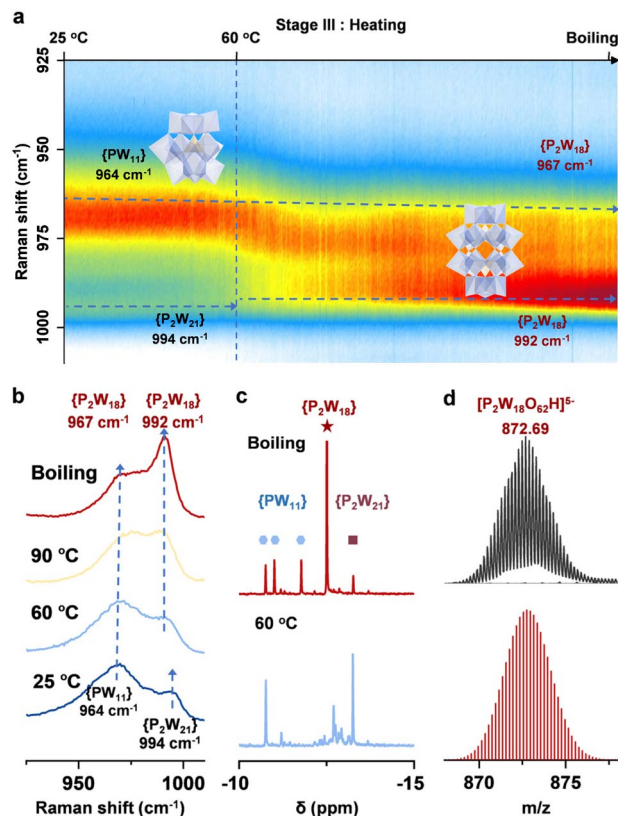
Fig. 3 (a) Stage III of heating: 2D Raman mapping (925 cm -1 to 1010 cm -1 ); (b) the corresponding Raman spectra at different temperatures; (c) 31 P NMR spectrum of the reaction solution at 60 °C and on boiling; (d) ESI-MS spectrum in negative ion mode of the solution after 24-hour reflux (the red and black lines represented simulated and experimental values, respectively).
