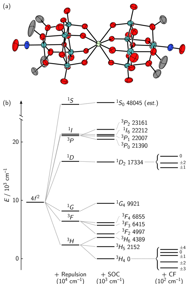
Fig. 1 (a) A 50% thermal ellipsoid plot of 1\text{-Pr} with the cations and hydrogens omitted for clarity. (b) The energies of all f\text{-}f transitions of a free atomic \text{Pr}^{\text{III}} ion are determined primarily by interelectron repulsion and SOC. 30,31 There are further CF splittings when \text{Pr}^{\text{III}} is in a molecule, here shown only for the {}^3\text{H}_4 and {}^1\text{D}_2 levels (CF splitting not to scale).
