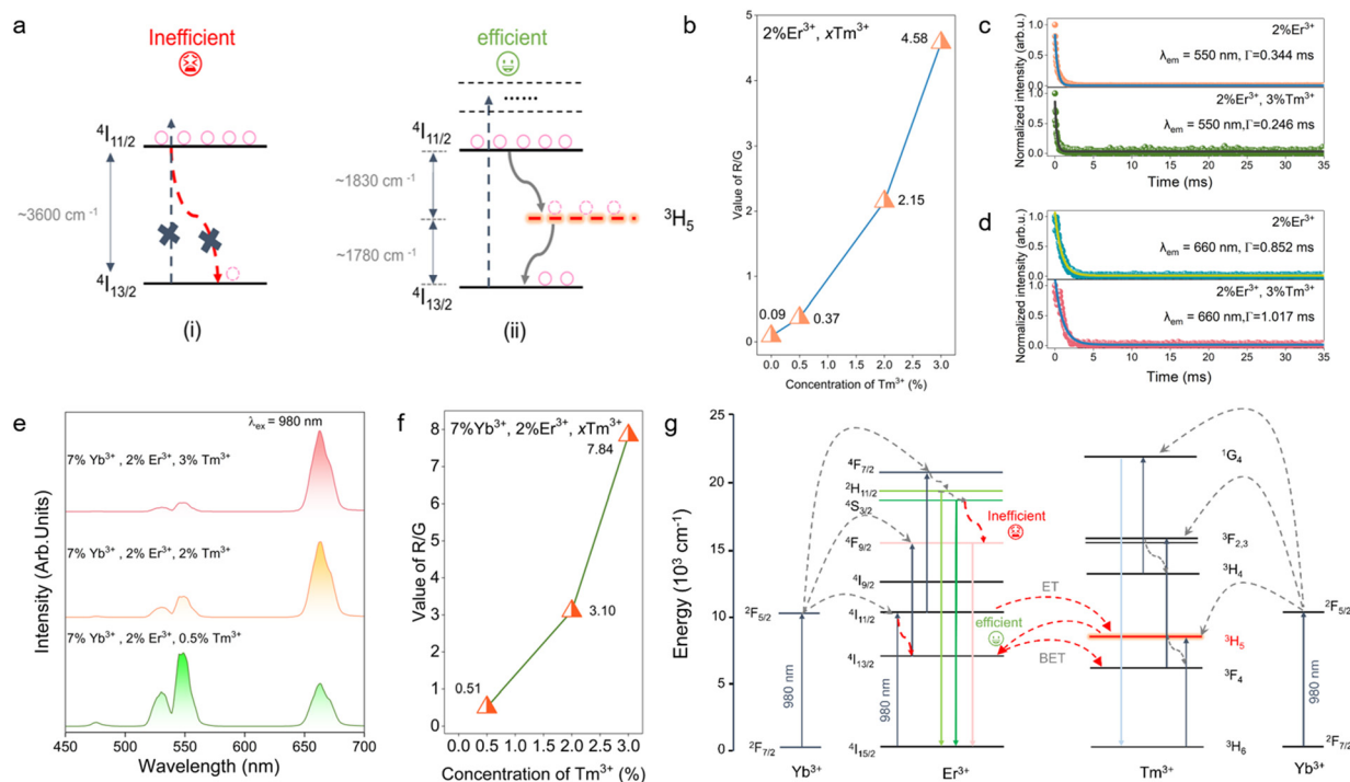
Fig. 2 (a) A schematic illustration of the regulatory role of the \text{Tm}^{3+} - {}^3\text{H}_5 energy level in UC emission of \text{Er}^{3+} . (b) R/G UC emission intensity ratio of GMTO: \text{Er}^{3+} , x\text{Tm}^{3+} ( x = 0 –3%) under 980 nm excitation. (c) UC decay lifetimes of green emission at 550 nm of \text{Er}^{3+} in the GMTO:2% \text{Er}^{3+} and GMTO:2% \text{Er}^{3+} , 3% \text{Tm}^{3+} under 980 nm excitation, respectively. (d) UC decay lifetimes of red emission at 660 nm of \text{Er}^{3+} in the GMTO:2% \text{Er}^{3+} and GMTO:2% \text{Er}^{3+} , 3% \text{Tm}^{3+} under 980 nm excitation, respectively. (e) UC emission spectra of GMTO:7% \text{Yb}^{3+} , 2% \text{Er}^{3+} , x\text{Tm}^{3+} ( x = 0.5 –3%) under 980 nm excitation. (f) R/G UC emission intensity ratio of GMTO:7% \text{Yb}^{3+} , 2% \text{Er}^{3+} , x\text{Tm}^{3+} ( x = 0.5 –3%). (g) Schematic of UC emissions of GMTO:Yb ^{3+} , Er ^{3+} , Tm ^{3+} upon 980 nm excitation.
