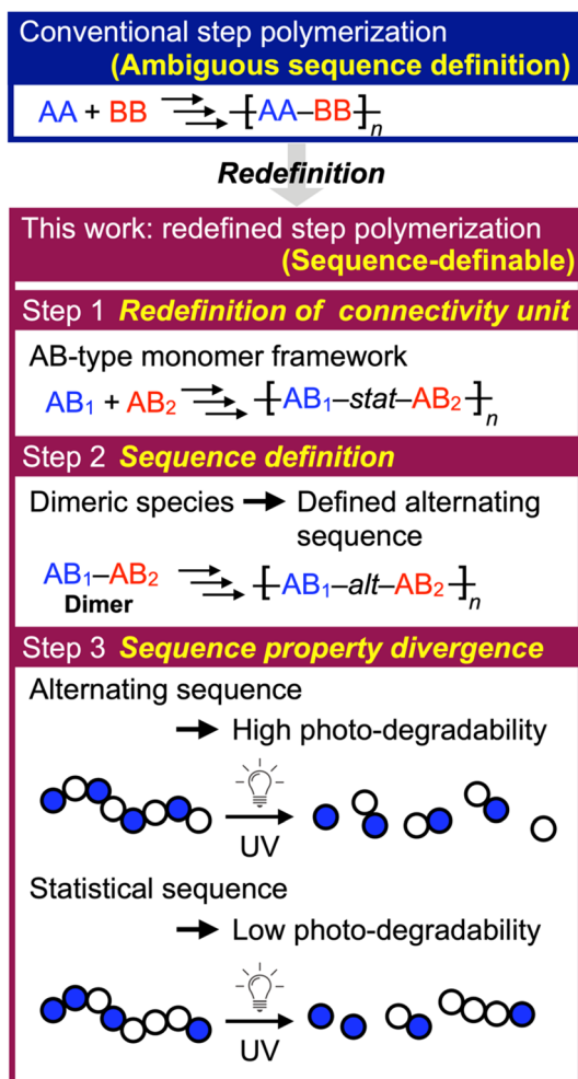
Fig. 8 Sequence definition of the polymer derived from step polymerization demonstrated in this work, highlighting sequence-property divergence for photo-degradation control.
