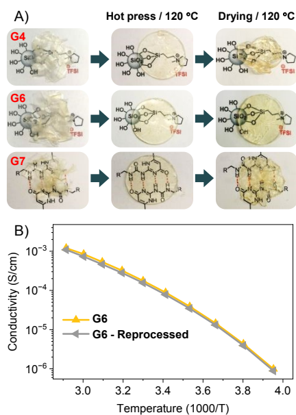
Fig. 6. A) Reprocessing of G4, G6 and G7 via hot-press at 120 °C for 3 hours; B) conductivity as a function of temperature of G6 before and after reprocessing.
