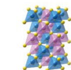
CuFeS 2 - chalcopyrite
