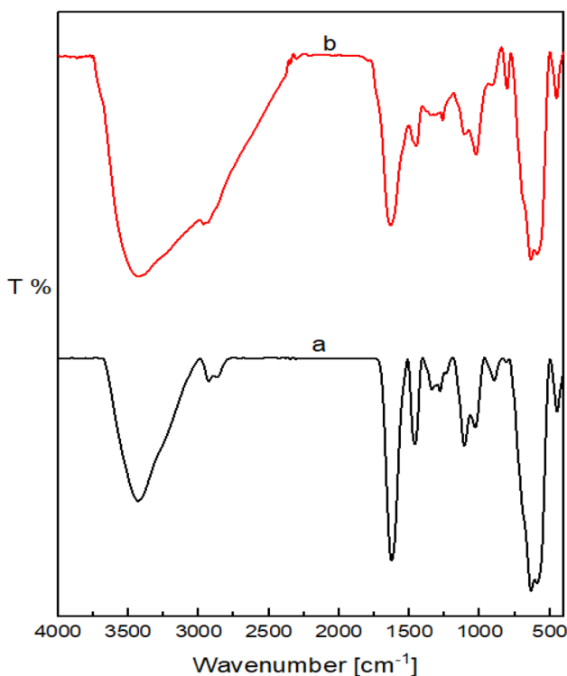
Fig. 9 FT-IR spectra of the fresh (a) and recovered Mag@RF/SB-Cu catalyst (b).
