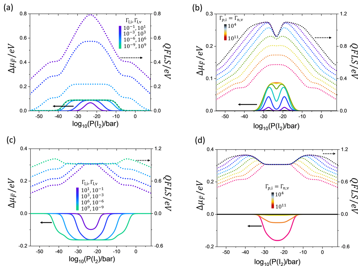
Fig. 8 Dependence of the ionic ( \Delta\mu_F ) and electronic (QFLS) change in chemical potential on the \Gamma_{Li}, \Gamma_{LV} , and \Gamma_{p,i}, \Gamma_{n,v} parameters, as a function of P(l_2) . Trends for (a) increasing h_{\text{ion}} > 0 ( \Gamma_{p,i} = \Gamma_{n,v} = 10^{11} ), (b) increasing \Gamma_{p,i} = \Gamma_{n,v} ( \Gamma_{Li} = 10^{-3}, \Gamma_{LV} = 10^3 ), (c) decreasing h_{\text{ion}} < 0 ( \Gamma_{p,i} = \Gamma_{n,v} = 10^{11} ), and (d) increasing \Gamma_{p,i} = \Gamma_{n,v} ( \Gamma_{Li} = 10^3, \Gamma_{LV} = 10^{-3} ). All remaining parameters are the same as the ones used in Fig. 3. h_{\text{ion}} = \log_{10}\left(\frac{\Gamma_{LV}}{\Gamma_{Li}}\right) .
