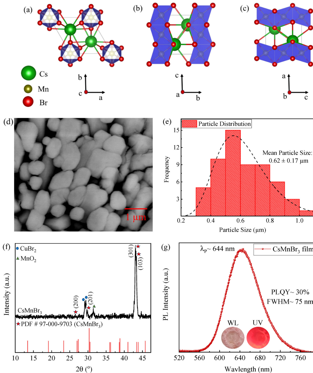
Fig. 2 Crystal structure of CsMnBr 3 projected along (a) c -axis, (b) a -axis, and (c) b -axis, (d) a SEM image of the as-prepared CsMnBr 3 film, (e) histograms depicting the distribution of particle sizes, (f) XRD spectra of the as-prepared CsMnBr 3 film, and (g) PL spectra of the as-prepared CsMnBr 3 film with the inset showing optical images of the film under white and UV light (~365 nm), respectively.
