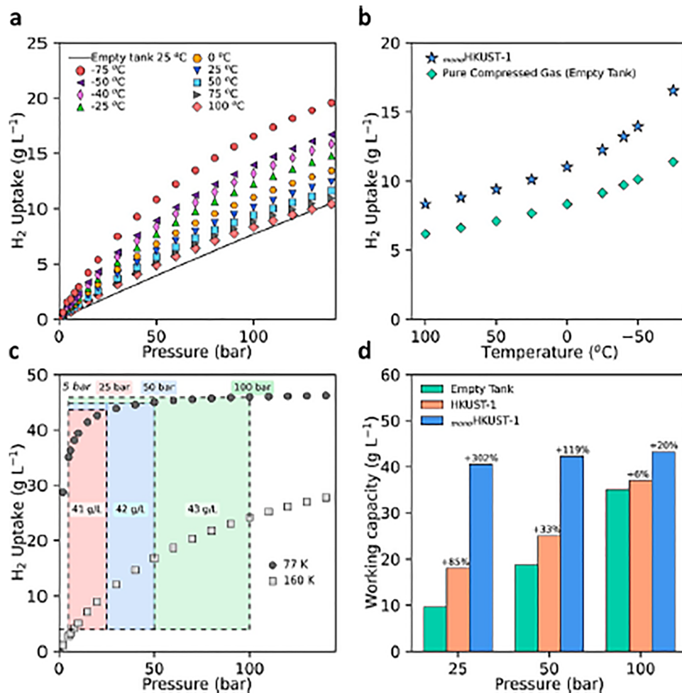
Fig. 28 (a) \text{H}_2 uptake of \text{monoHKUST-1} at different temperatures (b) volumetric storage of \text{monoHKUST-1} compared to compressed gas at 100 bars (c) \text{H}_2 delivery under cryogenic conditions and (d) deliverable \text{H}_2 capacity of \text{monoHKUST-1} compared to HKUST-1 powder and an empty tank at various adsorption pressures at 77 K. 31 Reproduced with permission from ref. 31. Copyright (2022) American Chemical Society.
