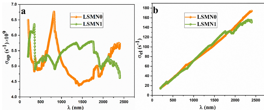
Fig. 12 (a) Spectral variation of optical conductivity \sigma_{op}(\lambda) . (b) Spectral variation of electrical conductivity \sigma_{el}(\lambda) for LSMN0 and LSMN1.
