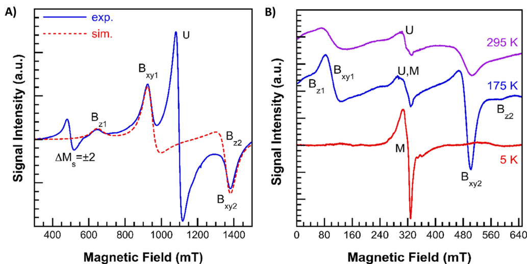
Fig. 6 EPR spectra of \text{RbCu}(\text{HCO}_2)_2\text{Cl} powder at (A) 33.9 GHz and 295 K and (B) 9.4 GHz at 295, 175 and 5 K. Dotted-red line in A is a simulation with the parameters indicated in the text.
