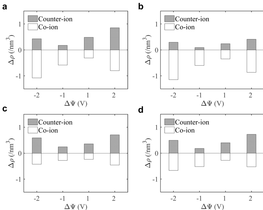
Fig. 4 Voltage-induced changes in ion population inside MXene pores. (a–d) Change in the equilibrium pore ion population, \Delta\rho = \rho(\Delta\psi) - \rho(0V) , in pores with widths of 0.7 nm (a), 0.8 nm (b), 1.0 nm (c), and 1.2 nm (d). The negative values indicate a decrease in the number of ions inside the pore.
