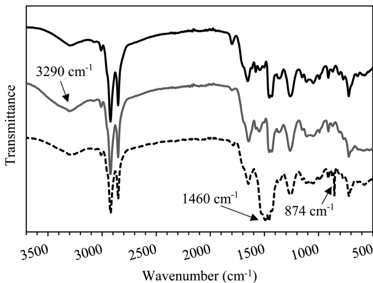
Fig. 6 IR spectra of FO-NIPU (black, top), deionized water NIPU (gray, middle), and sea water-exposed FO-NIPU (black dashed, bottom).
