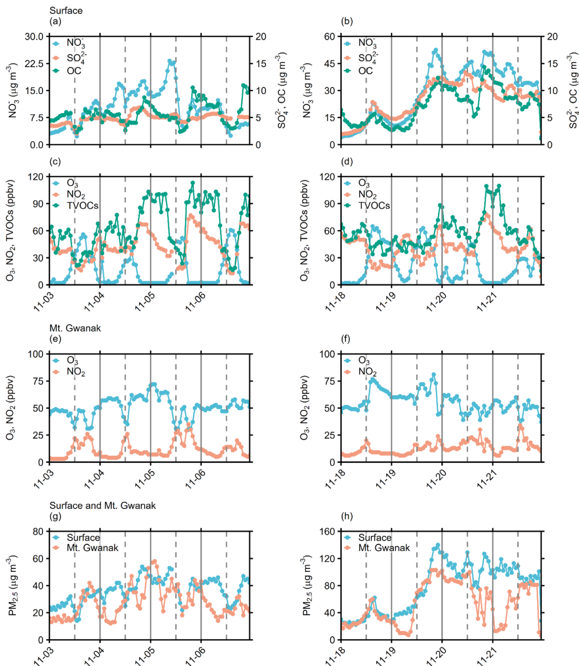
Fig. 5 Hourly variations of PM_{2.5} components and gaseous species during Cases 2 and 4. The left and right columns show Cases 2 and 4, respectively. (a–d) Surface-level concentrations of NO_3^- , SO_4^{2-} , OC, O_3 , NO_2 and TVOCs. (e and f) O_3 and NO_2 concentrations measured at the summit of Mt. Gwanak. (g and h) PM_{2.5} concentrations at the surface (Dongdaemun-gu site) and at the summit of Mt. Gwanak.
