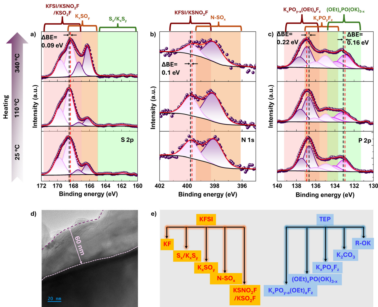
Fig. 4 (a)–(c) XPS spectra showing the interfacial chemistry of anodic decomposition products after the 4th cycle of potassiated graphite (fully charged to 4.3 V vs. \text{K/K}^+ ) at three temperatures: at 25 °C (bottom), 110 °C (middle) and 340 °C (top); (a) S 2p, (b) N 1s spectra; (c) P 2p spectra. Binding energy shifts indicate temperature-driven chemical changes. (d) TEM image of the potassiated graphite anode showing a SEI thickness of \sim 60 nm; (e) proposed electrochemical decomposition of KFSI and TEP contributing to SEI formation during cycling.
