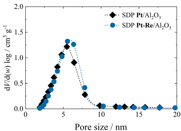
Fig. 5 Pore volume ( V_{\text{BHD}} ) and pore size distribution (PSD) obtained for Pt/ \text{Al}_2\text{O}_3 (0.3 wt% Pt) and Pt-Re/ \text{Al}_2\text{O}_3 (0.3 wt% Pt, 0.27 wt% Re, Re/Pt = 0.88) via \text{N}_2 physisorption obtained using the adsorption branch.
