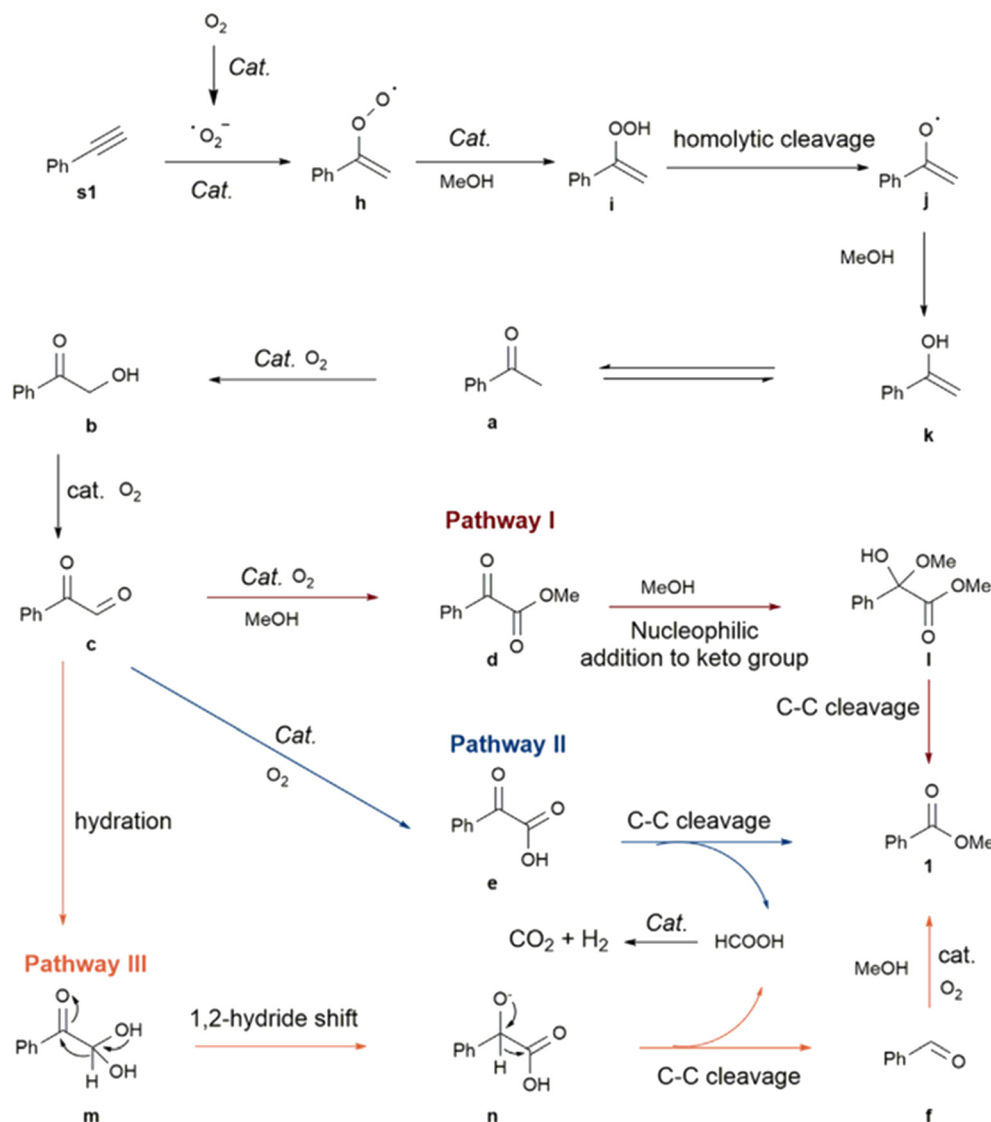
Fig. 20 Possible pathway for the oxidative esterification of alkynes. 239 Reproduced with permission from ref. 239. Copyright 2023 Elsevier.
