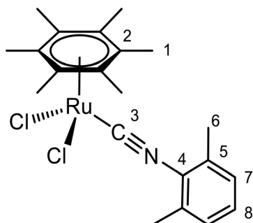
Chart 10 Structure of 2f (numbering refers to carbon atoms).
