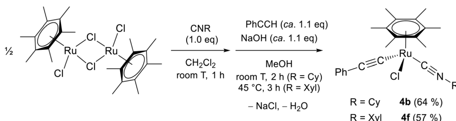
Scheme 3 Two-step synthesis of [RuCl(CCPH)(CNR)( \eta^6 -C 6 Me 6 )] from [RuCl 2 ( \eta^6 -C 6 Me 6 )], and the corresponding isocyanide, phenylacetylene and NaOH. Reactions were carried out under N 2 ; isolated yields in parentheses.
