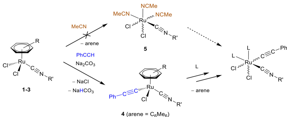
Scheme 6 Overview of the investigated reactivity of ruthenium(II) arene isocyanide complexes with excess \text{PhCCH} and \text{Na}_2\text{CO}_3 in MeCN ( \text{L} = \text{Cl}^- , solvent or other ligands).
