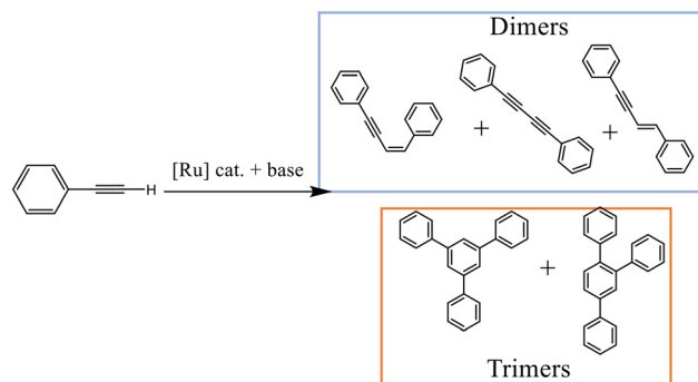
Scheme 5 Phenylacetylene dimerization/cyclotrimerization reaction and products.
