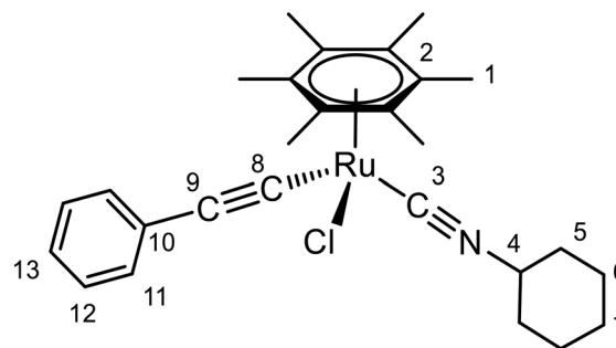
Chart 15 Structure of 4b (numbering refers to carbon atoms).
