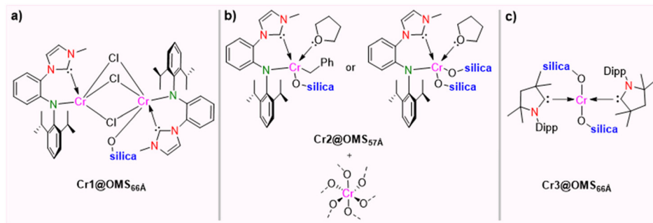
Fig. 6 Proposed structures for the immobilized Cr complexes a) Cr1@OMS 66A , b) Cr2@OMS 57A and c) Cr3@OMS 66A based on XAS analysis. Regarding Cr2@OMS 57A , the hexacoordinate chromium oxide species could not be characterized further and is therefore shown only schematically.
