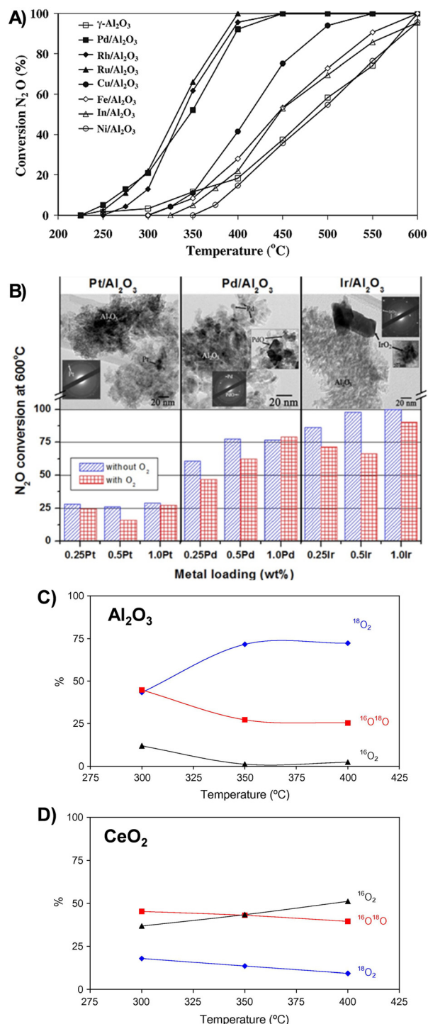
Fig. 4 (A) Comparison of catalytic activity for various \text{Al}_2\text{O}_3 -supported metal catalysts (2 wt% metal tested at a GHSV = 35 000 \text{h}^{-1} with P_{\text{N}_2\text{O}} = 0.12% and a balance in He). Reprinted from ref. 32 with permission from Springer Nature. (B) \text{N}_2\text{O} conversion at 600 ^{\circ}\text{C} with and without \text{O}_2 for Pt, Pd, and Ir on alumina catalysts with insight to surface morphology. Reprinted from ref. 33 with permission from Elsevier. Oxygen content produced from isotopic ^{15}\text{N}_2^{18}\text{O} pulse experiment on 0.5 wt% Rh on (C) \text{Al}_2\text{O}_3 and (D) \text{CeO}_2 to show the evolution of oxygen species, highlighting the oxygen donating role of the \text{CeO}_2 support. C and D Reprinted from ref. 27 with permission from Elsevier.
