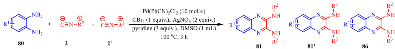
Scheme 40 Control experiment.
