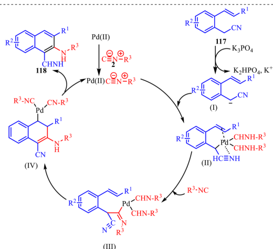
Scheme 62 Plausible mechanism synthesis of naphthalen-2-amine derivatives.
