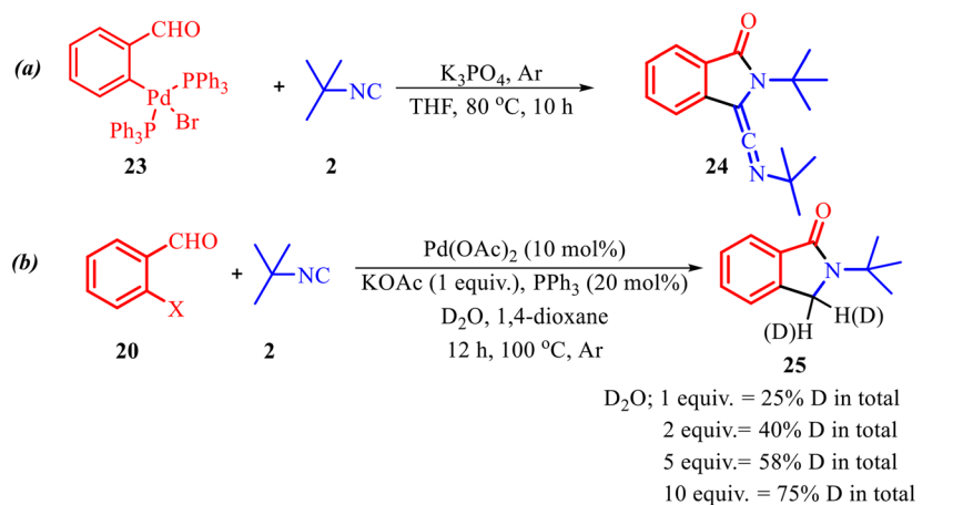
Scheme 10 (a) Determination of palladium complex formed in the reaction. (b) Determination of role of water in the reaction medium.
