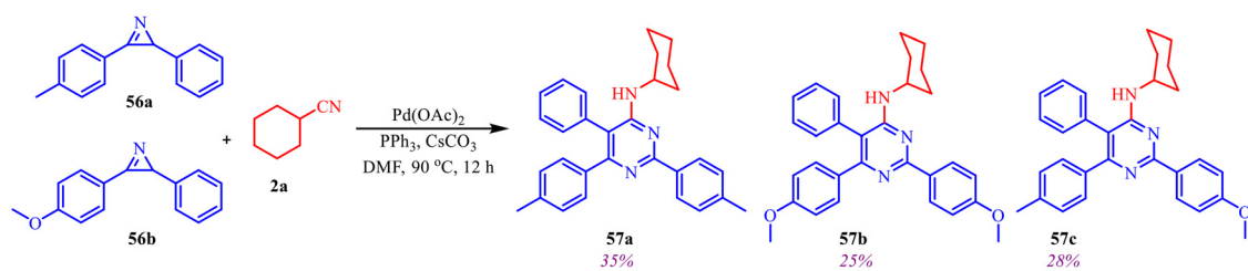
Scheme 27 Control reaction.
