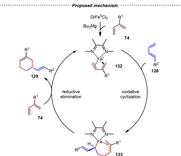
Scheme 29 Fe(II)/ \alpha -diimine-catalyzed asymmetric cross-[4+2] cycloadditions of unactivated 1,3-dienes.
