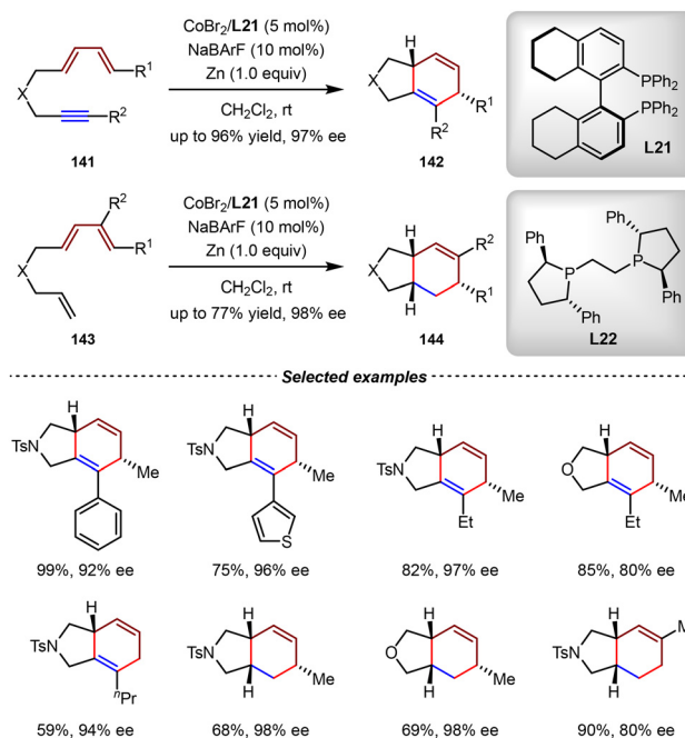
Scheme 31 \text{Co}(\text{I}) -catalyzed intramolecular [4+2] cycloaddition reactions of unactivated diene-yne and trienes.
