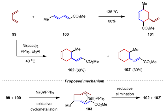
Scheme 25 Ni(0)/PPh 3 -catalyzed cross-[4+2] cycloadditions of 1,3-butadiene with methyl sorbate.
