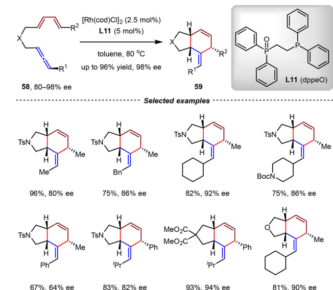
Scheme 17 Rh(I)/dppeO-catalyzed intramolecular [4+2] cycloadditions of optically active allenyl 1,3-dienes.
