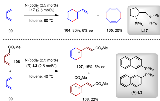
Scheme 26 Ni(0)-catalyzed asymmetric [4+2] cycloadditions of 1,3-dienes.
