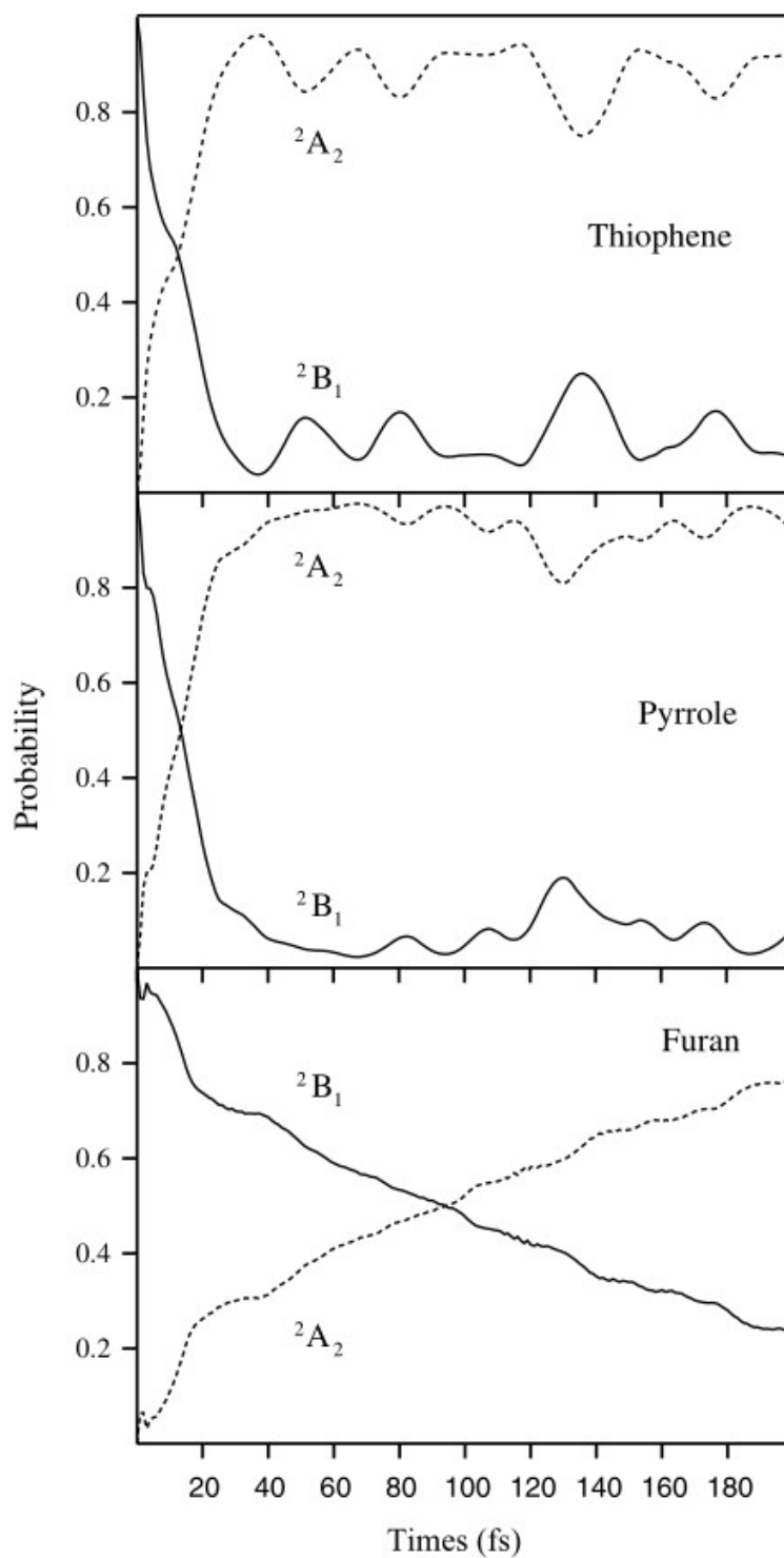
FIG. 8. Time-dependent electronic populations of the ^2A_2 and ^2B_1 electronic states of furan, pyrrole and thiophene cations for a broad band (vertical) excitation to the ^2B_1 electronic state in the centre of the Franck–Condon zone. Figure reproduced from Ref. [57] with permission from Elsevier, copyright 2004.
