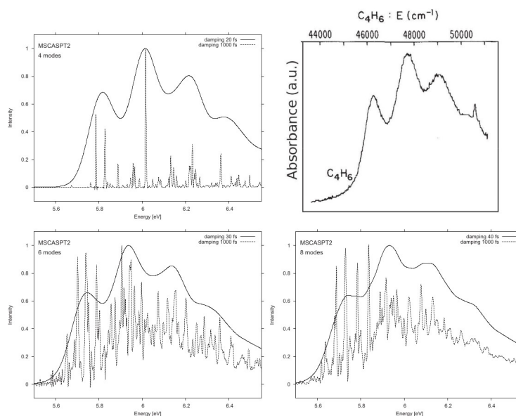
FIG. 6. Comparison of calculated spectra of butadiene with the experimental result by Vaida et al. [50]. The experiment is shown in the upper right panel. The dynamical results including 4 modes, 6 modes and 8 modes are depicted in the upper left, lower left and lower right panel, respectively. In all cases, \Delta E = 0.51 eV. Figure reproduced from Ref. [45]. with permission from Elsevier, copyright 2017.
