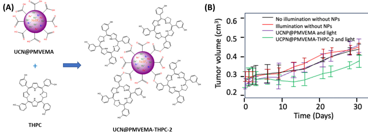
Fig. 6 (A) Structure of UCN@PMVEMA and UCN@PMVEMA-THPC-2. (B) In vivo PDT with UCN@PMVEMA-THPC-2. Tumour growth ( n = 4 ). Illumination was performed at 980 nm laser 10 min after administration. Statistical significance between UCN@PMVEMA-THPC-2 and other three groups p < 0.05 .
