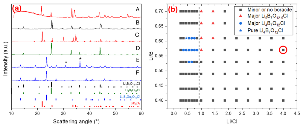
Fig. 2 (a) Powder XRD patterns (post-crystallization) of an aluminum-doped sample melted at 1150 °C for 30 minutes without cover (A), an undoped, unmelted boracite sample after sintering at 700 °C (B), an undoped sample melted at 950 °C without cover melted by itself in the furnace (C), an undoped sample melted at 950 °C without cover melted with 63 other samples in the furnace (D), a Ga-doped ( x = 2 ) sample melted at 950 °C with 7 other similar samples under a small boat (E), a Ga-doped ( x = 2 ) sample melted at 1000 °C by itself under a singular small crucible (F). (b) The phase diagram obtained with two batches of samples (separated by the dashed line) where each composition is the dispensed composition. The red circle indicates the target composition Li 4 B 7 O 12 Cl. All samples in the phase diagram on one side of the dashed line were melt-quenched together from 950 °C without covering the samples in the furnace.
