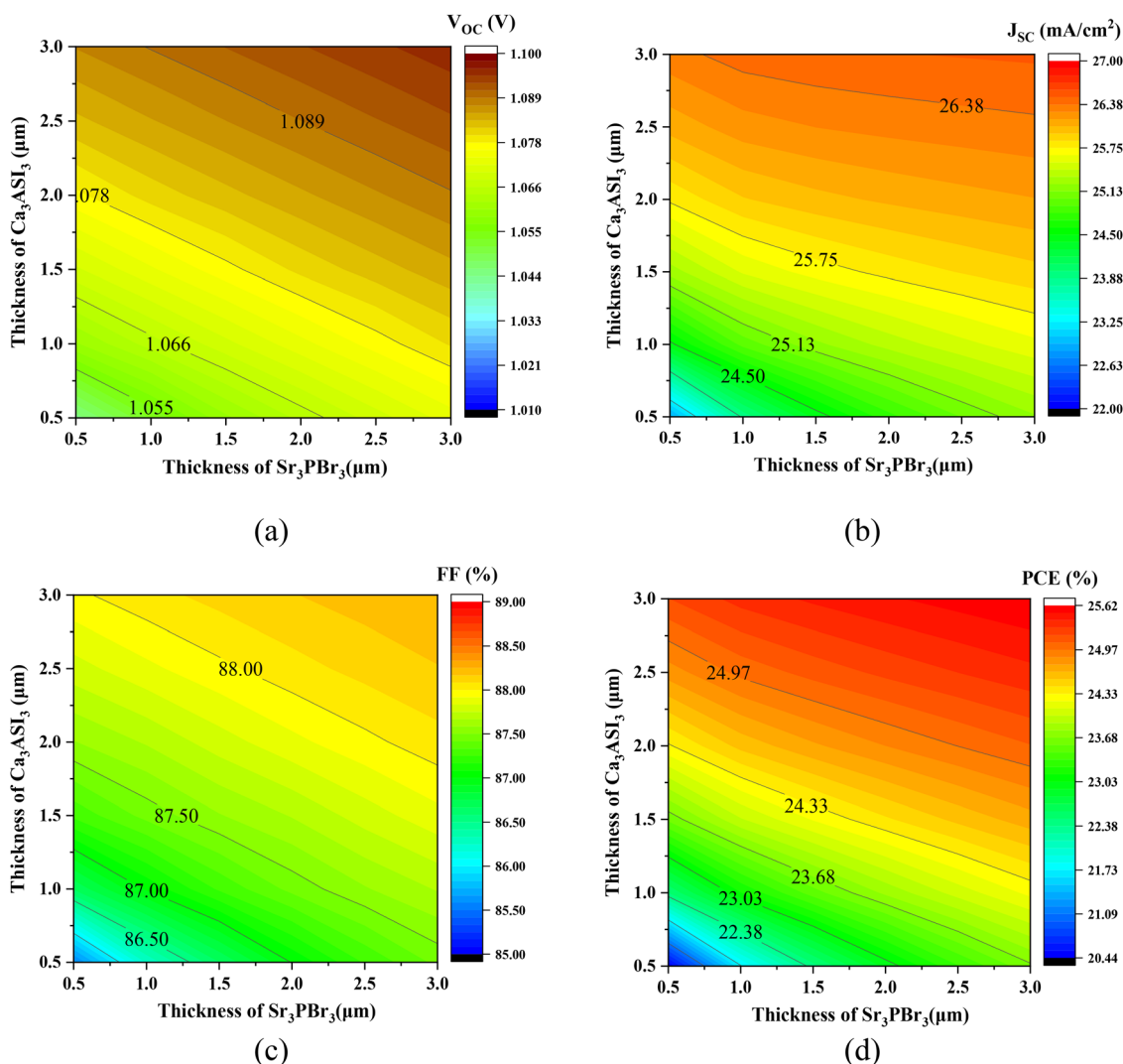
Fig. 3 Role of thickness variation of Sr 3 PBr 3 and Ca 3 AsI 3 (device-iii) on the photovoltaic parameters, (a) V_{OC} , (b) J_{SC} , (c) FF, and (d) PCE.
