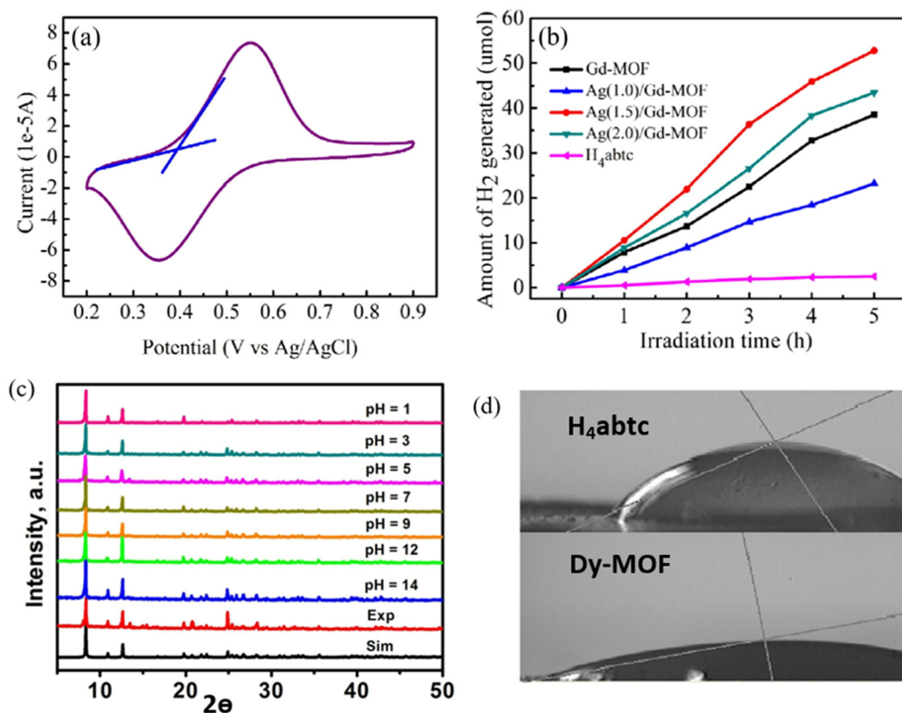
Fig. 9 (a) CV curves of the Gd-MOF. (b) Photocatalytic \text{H}_2 production under UV-Vis light irradiation over \text{H}_4\text{abtc} , Gd-MOF and Ag(X)/Gd-MOF. Reprinted with permission from ref. 175. (c) The pH stability of the dye-based Dy-MOF. (d) The differences in hydrophilicity between the dye-based Dy-MOF and \text{H}_4\text{abtc} ligand using contact angle measurements. Reprinted with permission from ref. 176. Copyright 2015 Royal Society of Chemistry.
