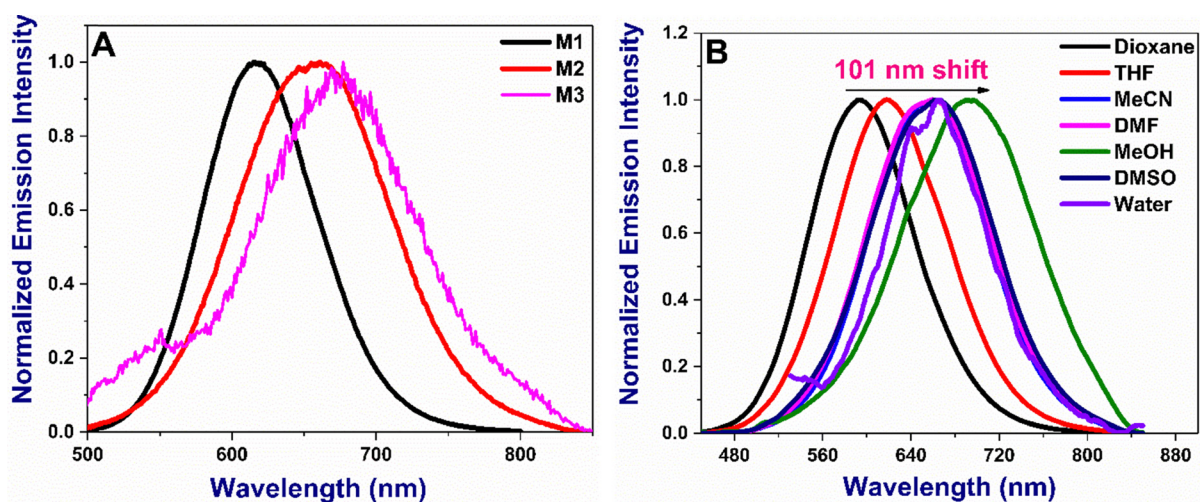
Fig. 3 (A) Normalized emission of all M1–M3 in acetonitrile (B) emission spectra of M2 in various solvents. Concentration: 10 \mu\text{M} . Emission spectra of M1 and M3 are given in Fig. S2 (ESI \dagger ).
