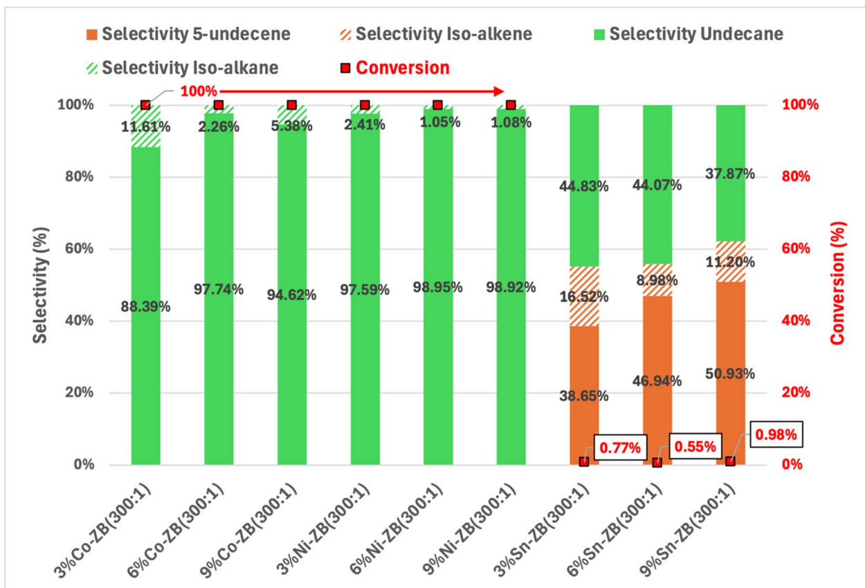
Fig. 12 Conversion and selectivity of all ZB(300 : 1) catalysts. Green = undecane and isomers associated. Orange = undecene and isomers associated. Blue = 6-undecanol and isomers associated.
