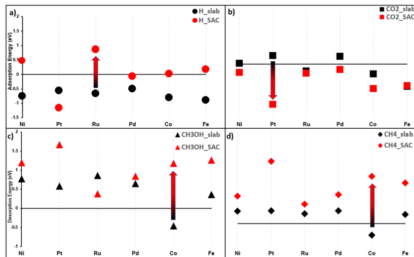
Fig. 5 Adsorption energies of: (a) H and (b) CO 2 on a slab and SAC, for the six chosen transition metals. Similarly, desorption energies of: (c) CH 3 OH and (d) CH 4 . Arrows show the biggest difference between the slab and SAC for each sub-figure.
