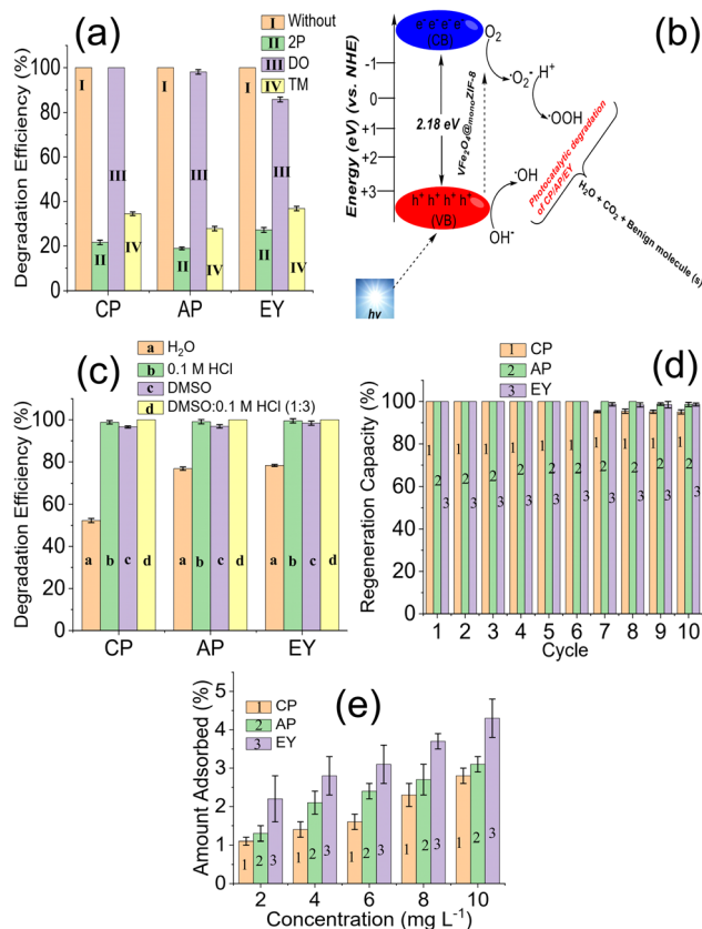
Fig. 4 Degradation efficiency of \text{VF}_2\text{O}_4@_{\text{monoZIF-8}} towards CP, AP and EY with and without ROS scavengers (a), proposed mechanism for the photodegradation of CP, AP and EY by \text{VF}_2\text{O}_4@_{\text{monoZIF-8}} (b), photodegradation efficiency of \text{VF}_2\text{O}_4@_{\text{monoZIF-8}} after treatment with different solvent systems (c), regeneration capacity of \text{VF}_2\text{O}_4@_{\text{monoZIF-8}} towards CP, AP and EY in different treatment cycles (d) and amounts of CP, AP and EY adsorbed by \text{VF}_2\text{O}_4@_{\text{monoZIF-8}} in the absence of light (e).
