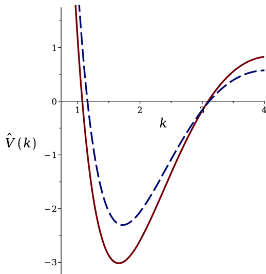
Fig. 2 The interaction potential times the pair distribution function in Fourier representation, \hat{V}(k) . Red solid line: u_{hs} = u_{hs}^+ (hard spheres). Blue dashed line: u_{hs} = u_{hs}^s (eqn (4), nearly hard spheres) k is in \sigma^{-1} units, and \hat{V}(k) is in arbitrary \epsilon units.
