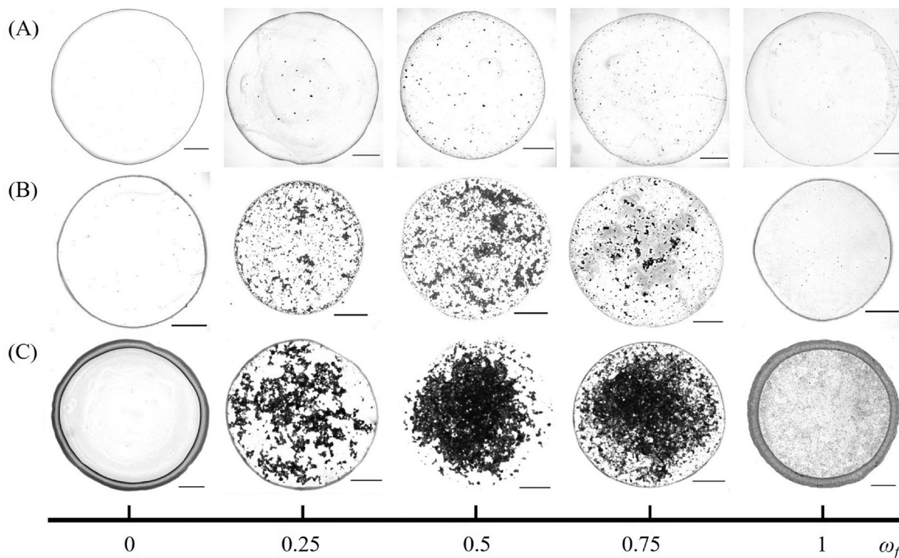
Fig. 1 Optical microscopy images of the dried deposit patterns formed by drying binary dispersions drops containing PS^+ - PS^- ( \approx 200 nm diameter) at (A) C_T = 0.01\% , (B) C_T = 0.1\% , and (C) C_T = 1\% for various mixing fractions ( \omega_f ). The microscopy images shown have been recorded soon after complete evaporation of the liquid from the sessile drops, which had a typical lifetime of about 10 min. Scale bar = 500 \mu\text{m} .
