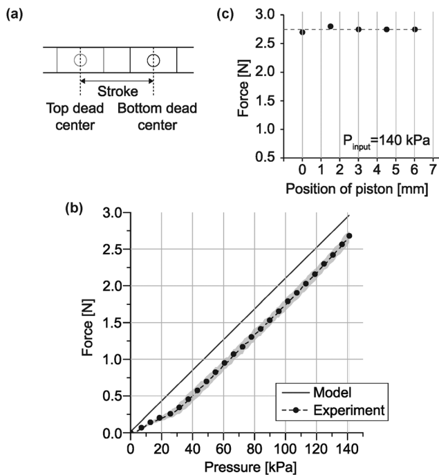
Fig. 5 The characterization of the actuator. (a) Schematic of the working range of the actuator. (b) Results of the blocked force experiment at the bottom dead center under increasing pressure. The dotted and dashed line indicates the average, while the shaded region represents the standard deviation. (c) Results of the block force experiment across the entire stroke at a constant pressure of 140 kPa.
