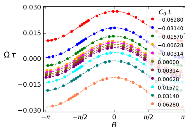
Fig. 6 Rotational velocity with spontaneous curvature. Variation of \Omega \tau as a function of \theta for various values of spontaneous curvature, with \alpha = 0.4 . The peak value, \Omega(0)\tau , increases with decreasing C_0 L < 0 and decreases with increasing C_0 L > 0 .
