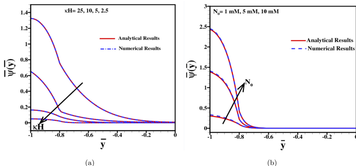
Fig. 13 Scaled potential distributions \bar{\psi}(\bar{y}) are shown as a function of scaled spatial coordinate \bar{y} for various values of (a) \kappa H ( = 2.5, 5, 10, and 25 ) with fixed N_0 = 1 mM and (b) N_0 ( = 1 mM, 5 mM, and 10 mM) with fixed \kappa H = 25 . Other model parameters are H = 25 nm, \delta = 5 nm, \bar{\sigma} = 2 , \epsilon_R = 0.1 , and r = 3.3 Å, respectively.
